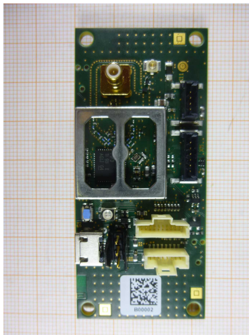
Photo 2: Shielding removed
