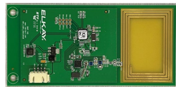
Filter NFC Board w/trace antenna
