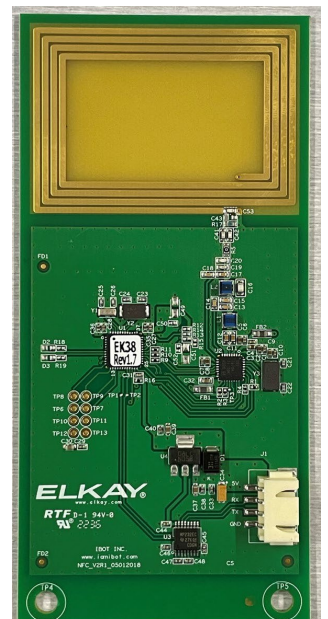
Filter NFC Board w/trace antenna
