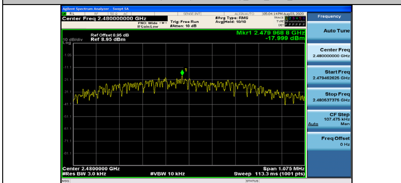
Maximum Peak power spectral density_BLE_2480_1M
