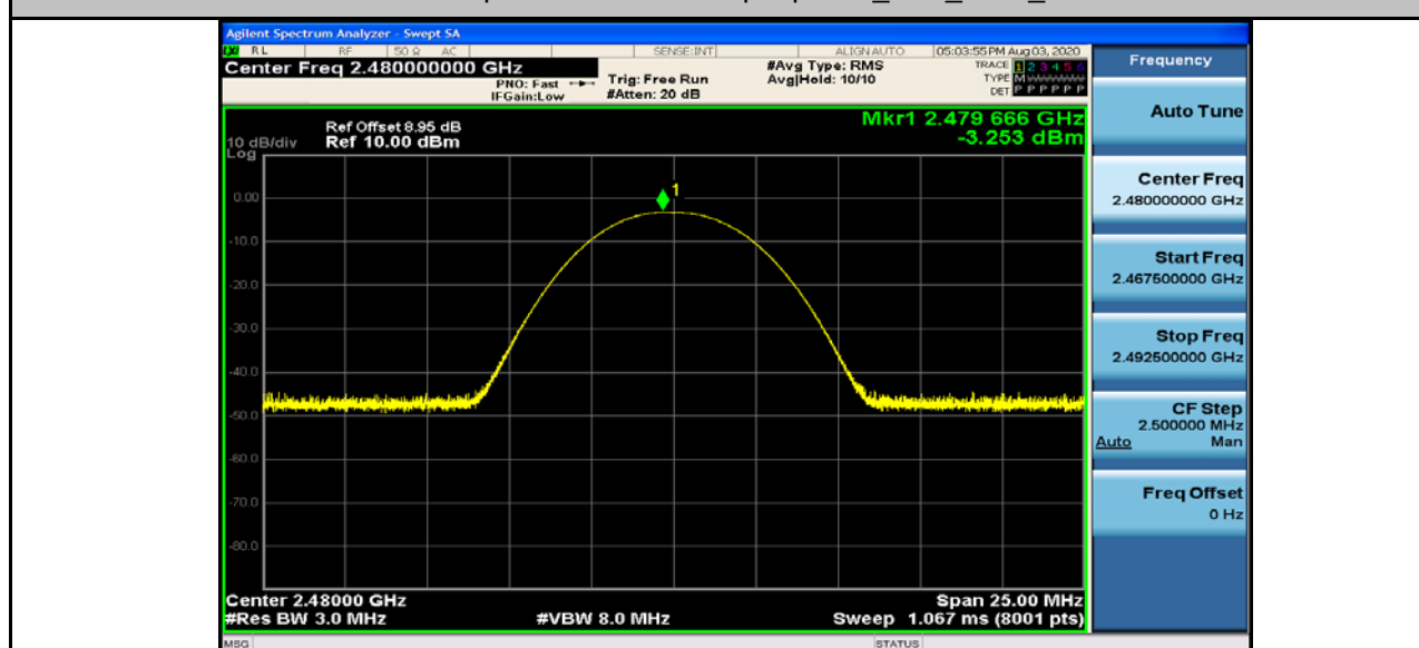
Maximum peak conducted output power_BLE_2480_1M
