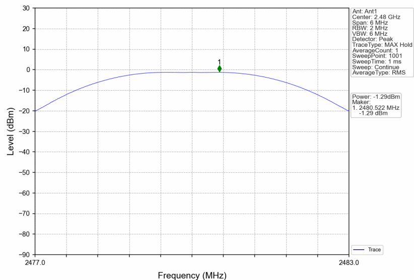
2M_HCH_2480MHz_Ant1_NTV
