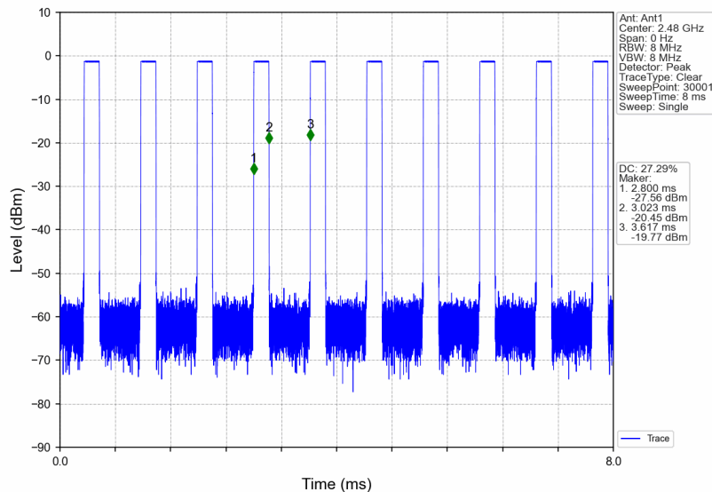
2M_HCH_2480MHz_Ant1_NTV
