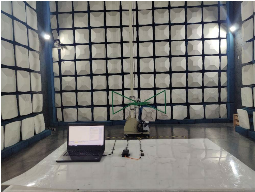
Radiated Spurious Emissions Test Setup 30MHz to 1GHz
