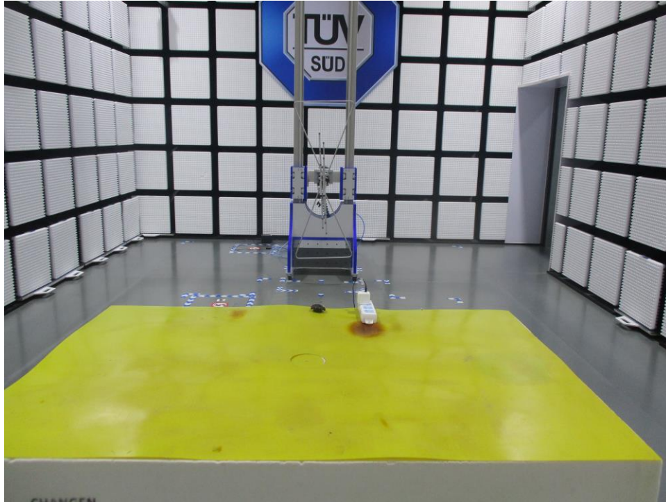
30M-1000MHz Radiated spurious emission
