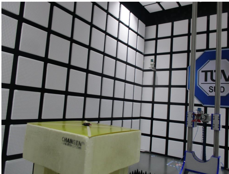
1G-18GHz Radiated spurious emission
