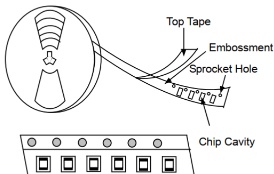
Embossed Tape
