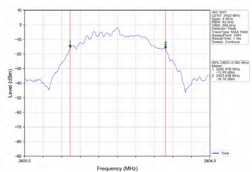
2M_LCH_2402MHz_Ant1_NTNV
