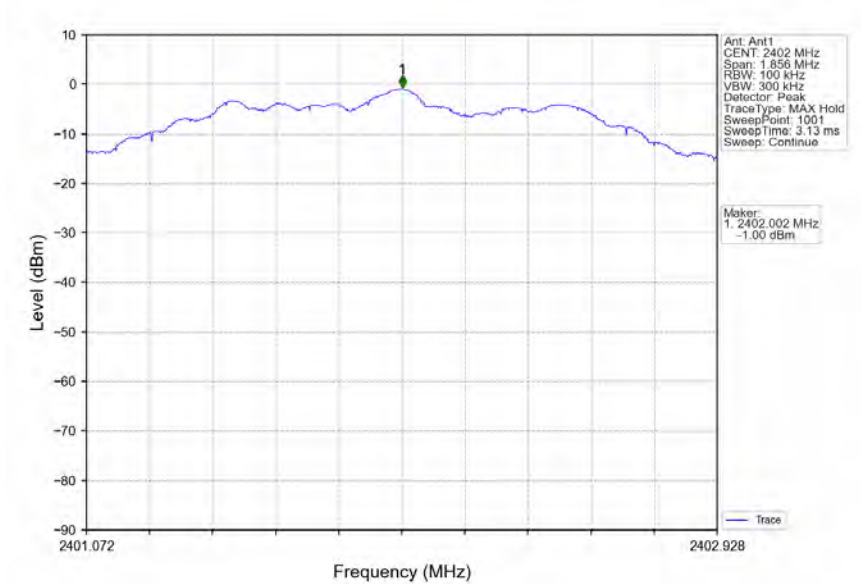
2M_LCH_2402MHz_Ant1_NTNV
