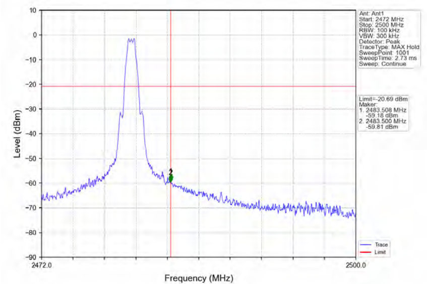
1M_HCH_2480MHz_Ant1_NTNV
