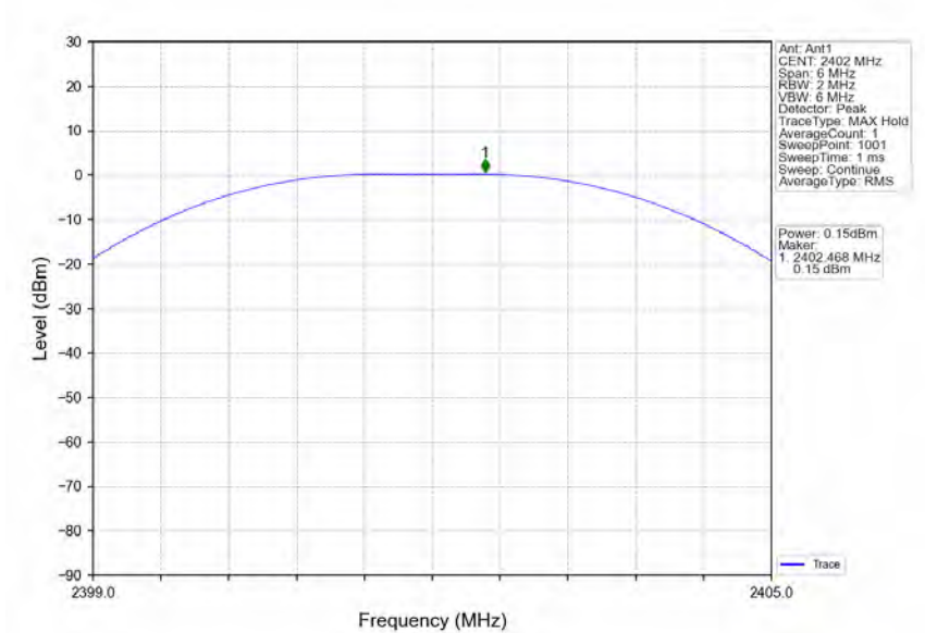
2M_LCH_2402MHz_Ant1_NTNV
