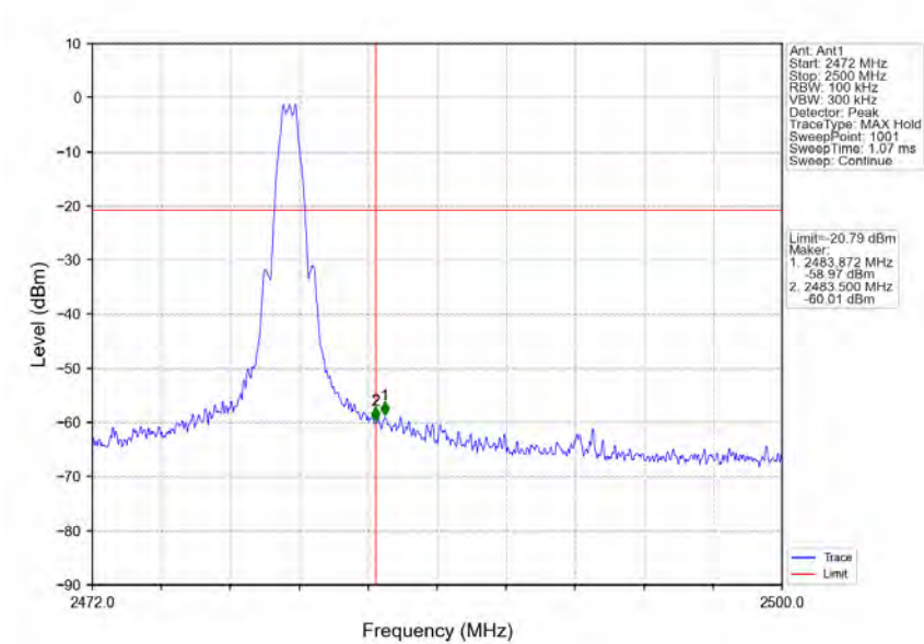
1M_HCH_2480MHz_Ant1_NTNV
