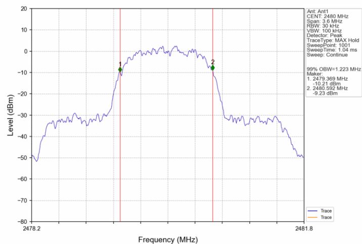
8DPSK 3DH5_HCH_2480MHz_Ant1_NTNV
