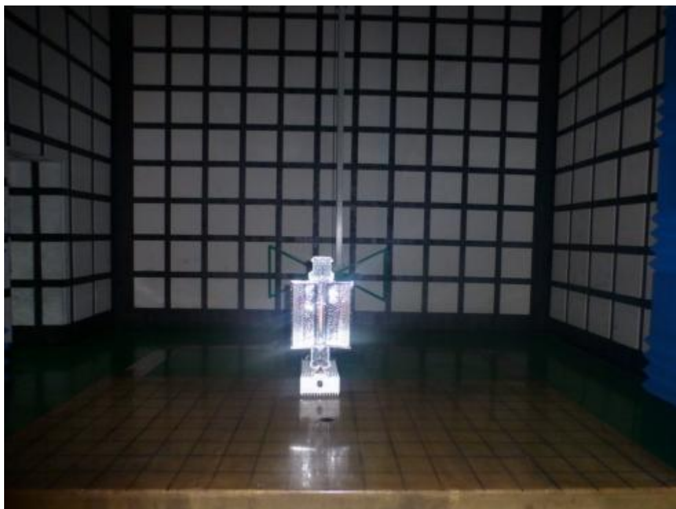
Radiated Emission (30MHz -1GHz) Setup photo
