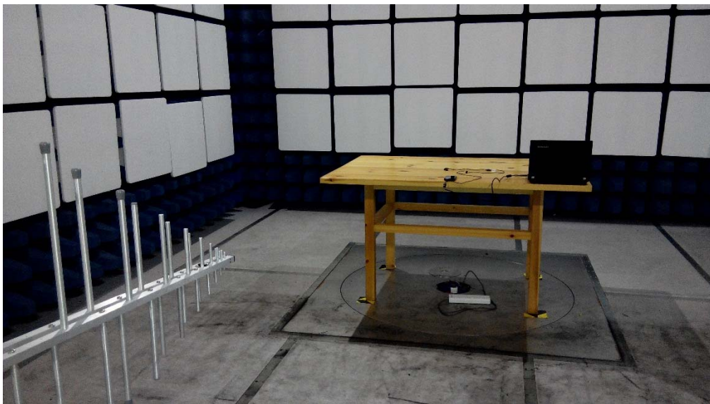
30MHz~1GHz USB Mode
