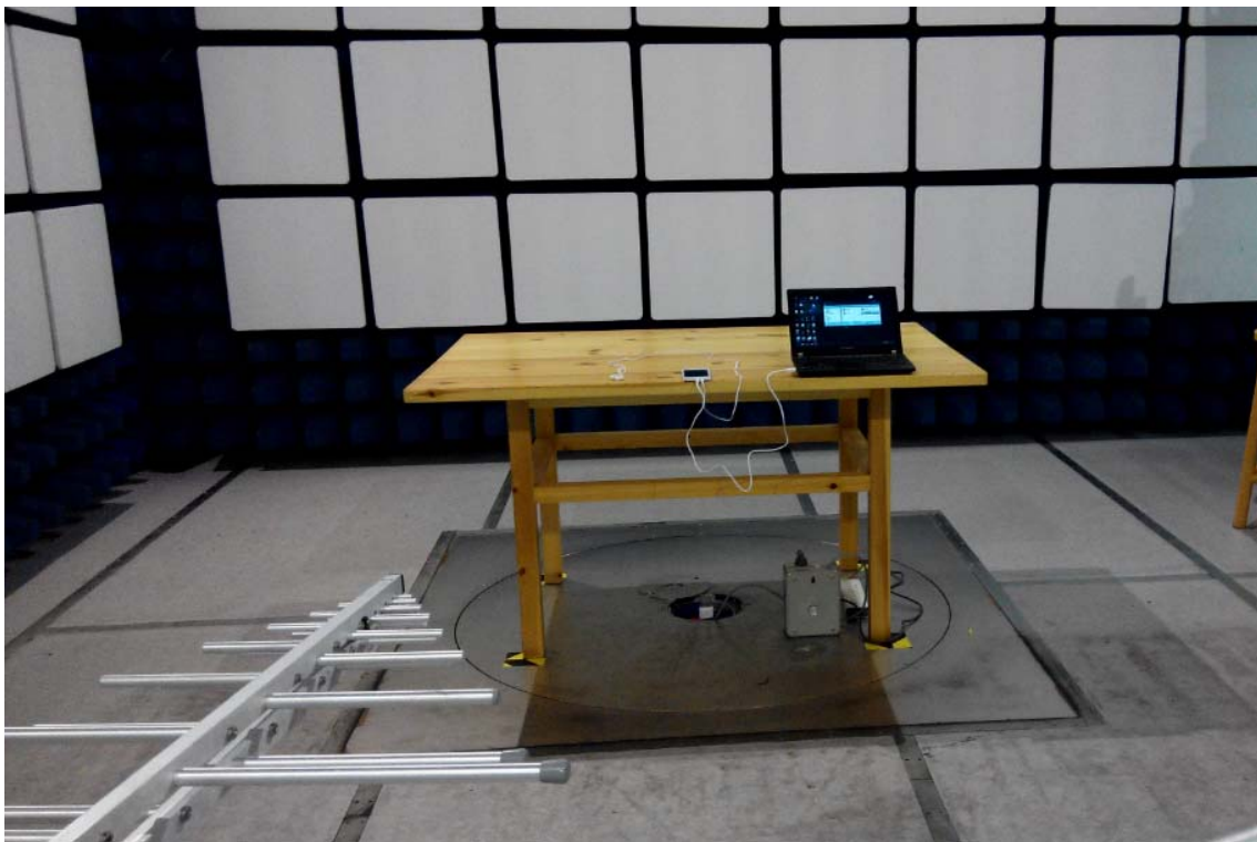
30MHz-1GHz (USB MODE)
