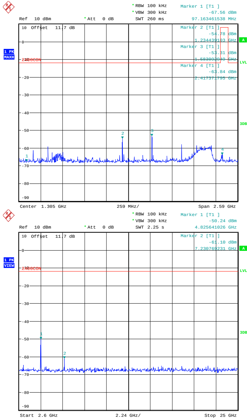
Plot 5.4.4.2.1. Conducted Spurious Emissions, 20MHz Ch Spacing, 2412 MHz, BPSK Modulation, 10 MHz – 25 GHz
