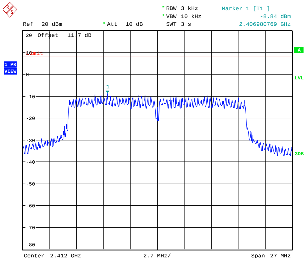
Plot 5.6.4.1. Power Spectral Density, BPSK Modulation, Channel #1, 2412 MHz
