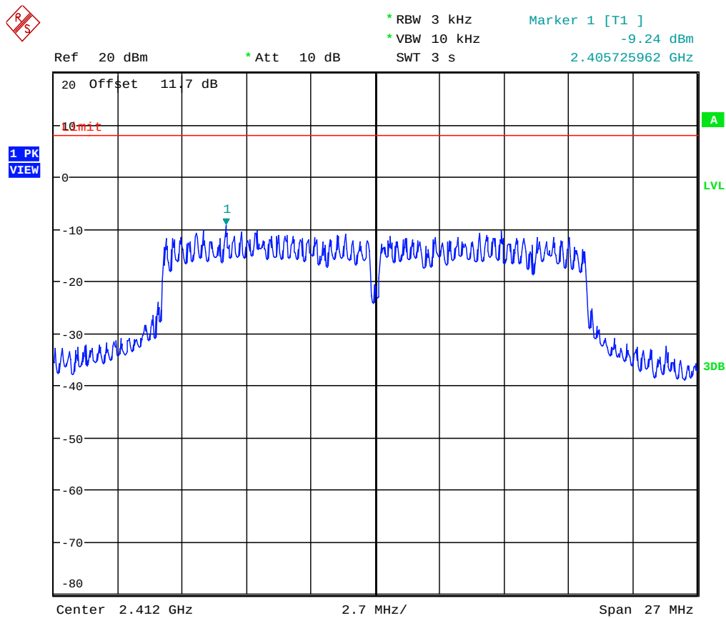
Plot 5.6.4.7. Power Spectral Density, 16-QAM Modulation, Channel #1, 2412 MHz
