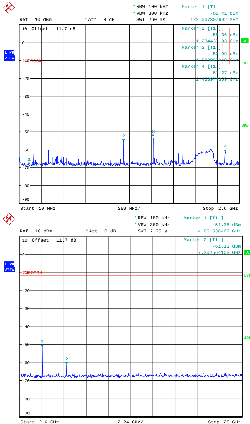
Plot 5.4.4.2.2. Conducted Spurious Emissions, 20MHz Ch Spacing, 2437 MHz, BPSK Modulation, 10 MHz – 25 GHz
