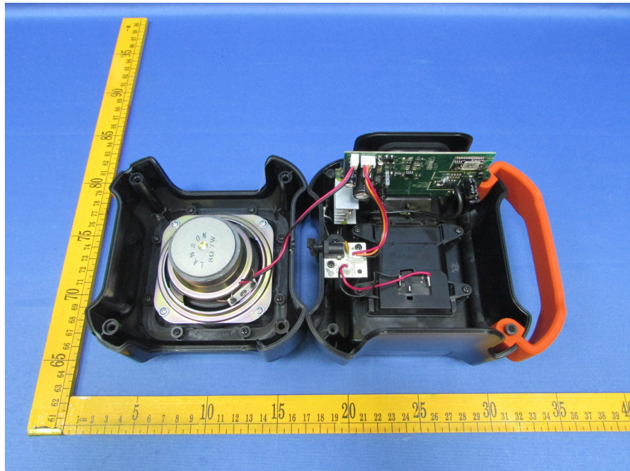
BDBTS20 & BDBTS20B
