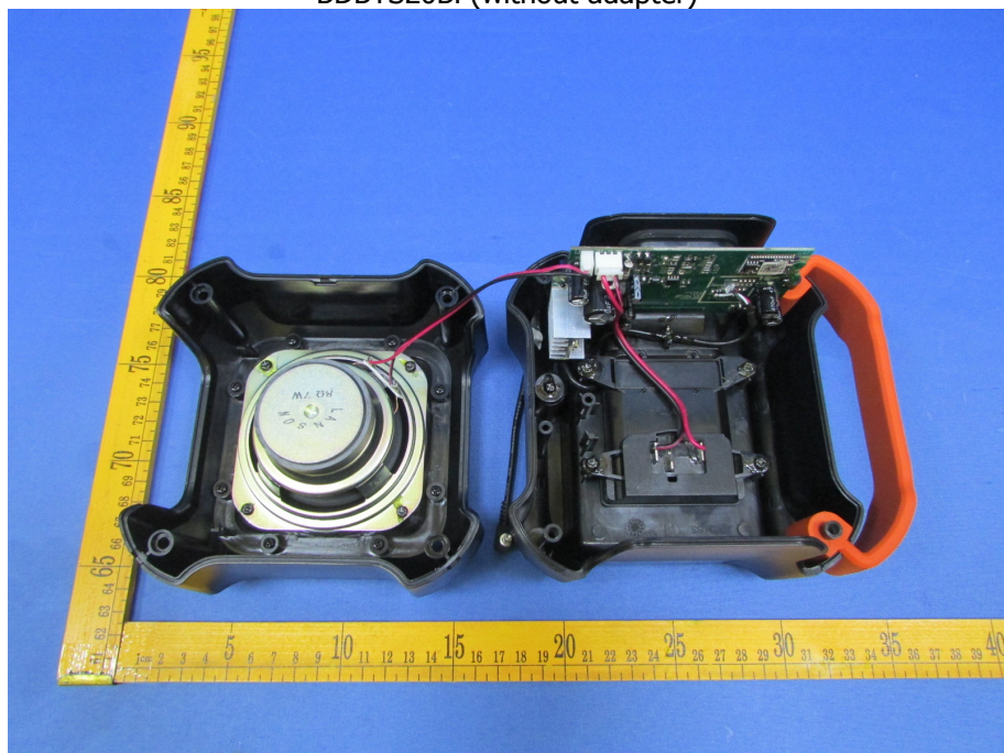
BDBTS20BP(without adapter)
