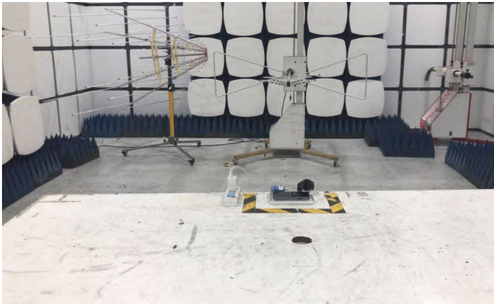
Photo of Radiation Emission Test
