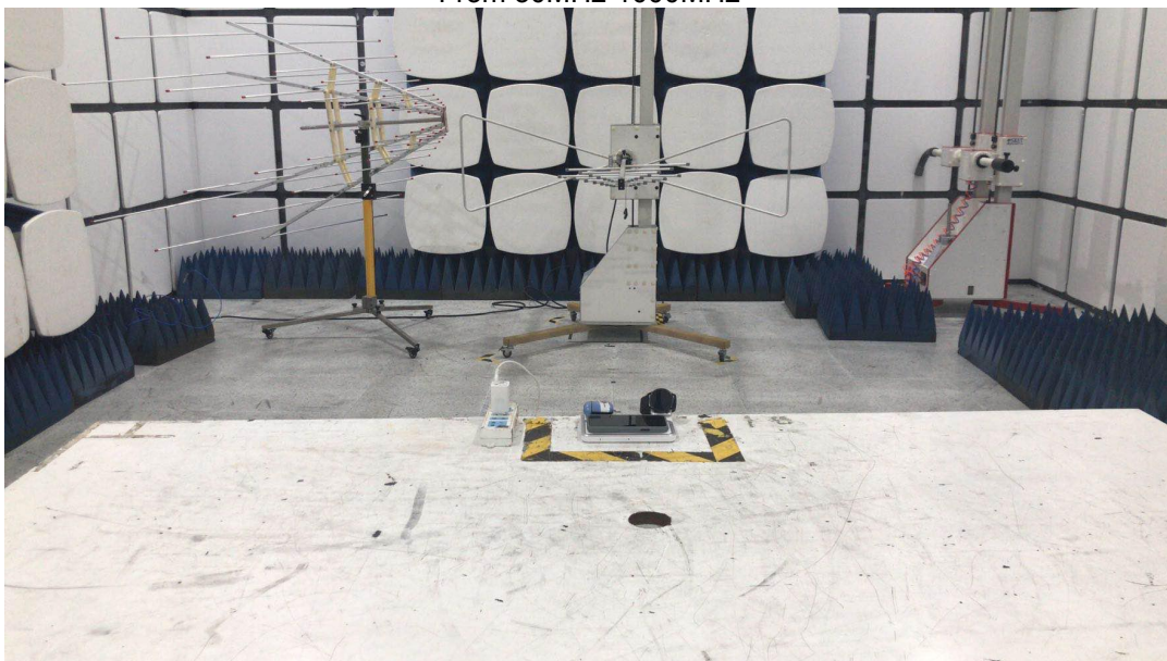
Radiated Spurious Emissions From 30MHz-1000MHz
