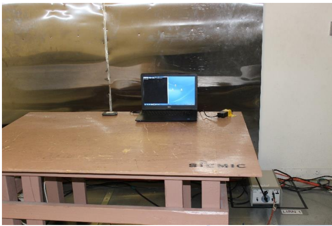
Conducted Emissions – Front View
