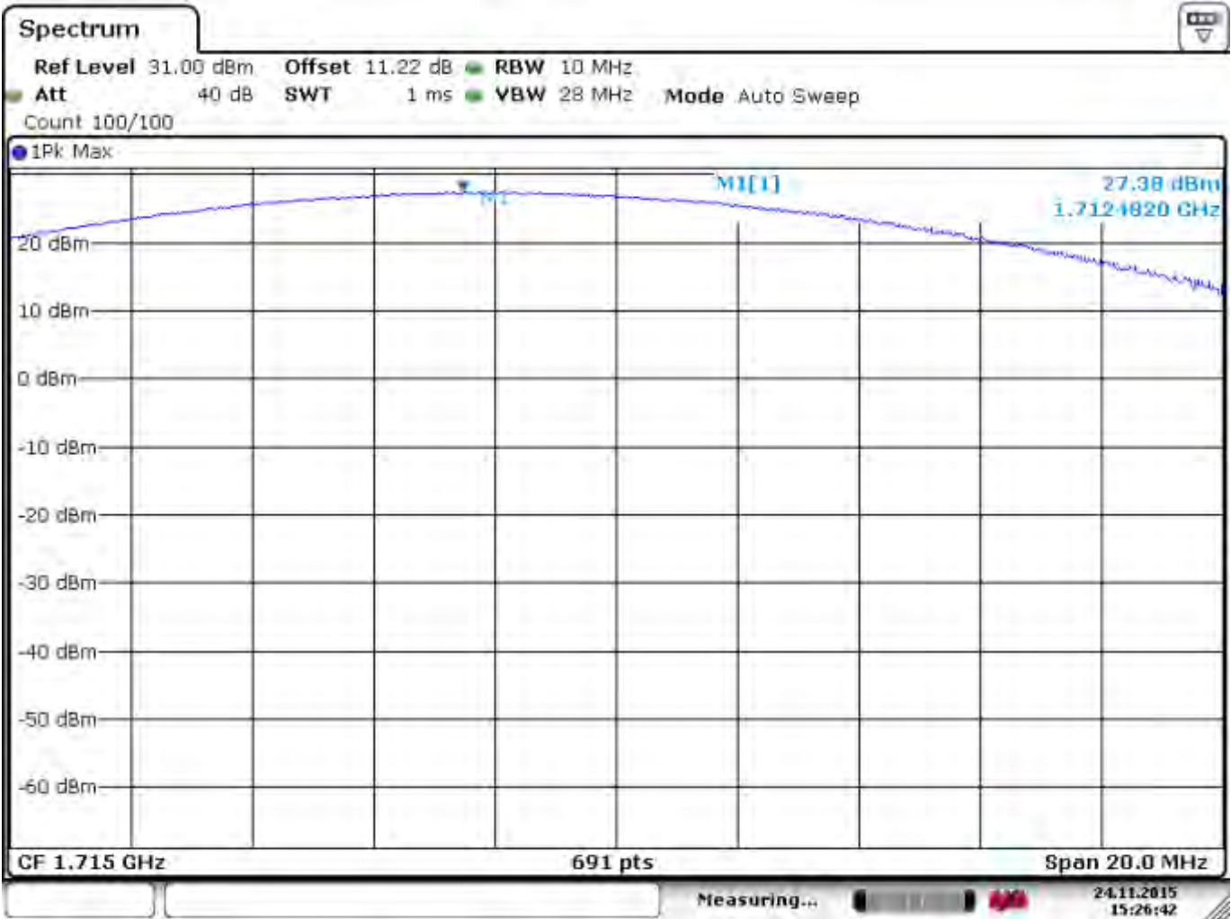
6.2.5.5.2 Figure 25 Pk Pwr Band 4 Lo 10
