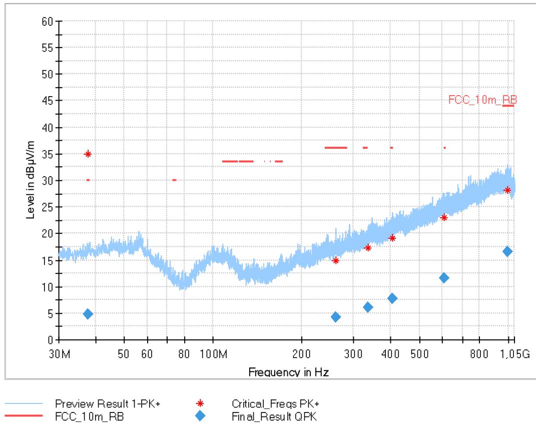
Plot 4: 30 MHz to 1 GHz, TX mode, vertical & horizontal polarization, 2 Msps, valid for all channels
