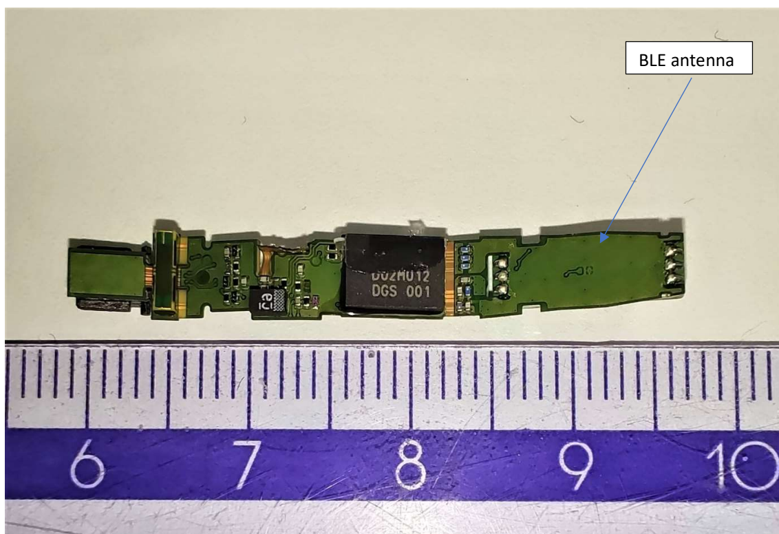
PCB showing the connector side
