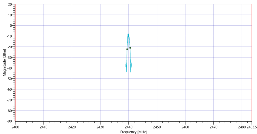
Plot_FCC Part 15.247 Bandwidth 99PCT-20dB ~ BT LE 1 Msps_06072021_100729.png
