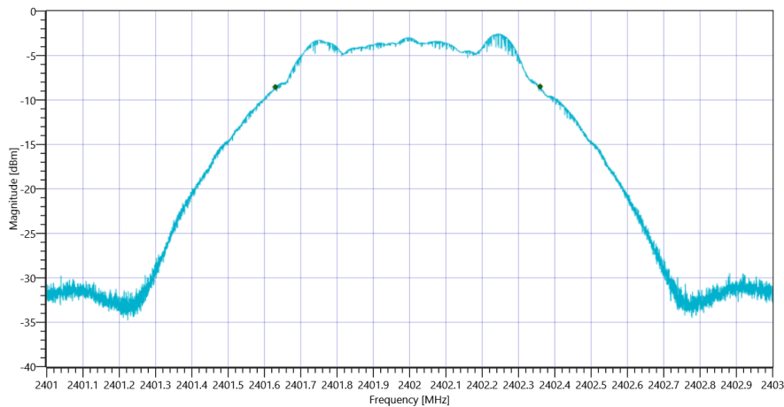
Plot_FCC Part 15.247 Maximum Peak Conducted Output Power DTS ~ BT LE 1 Msps DTS BW_06072021_095718.png
