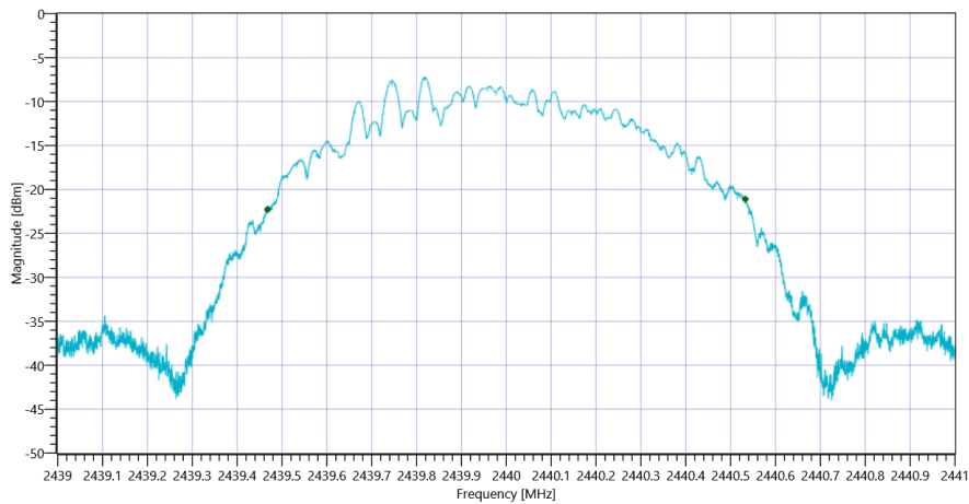
Plot_FCC Part 15.247 Bandwidth 99PCT-20dB ~ BT LE 1 Msps 99PCT_06072021_100722.png
