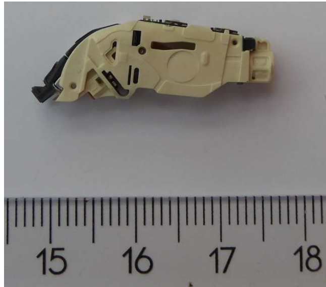
Radio module from the side
