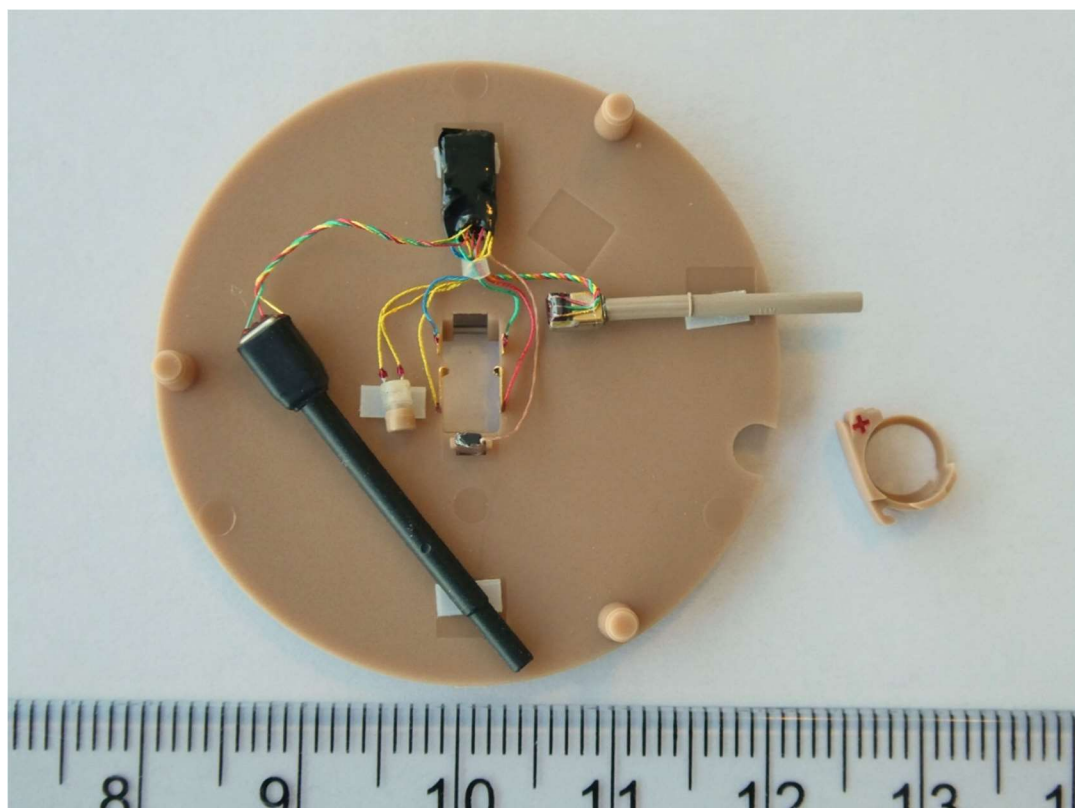
The AM_AU5_KIT10 hearing aid module stack up faceplate, front and back
