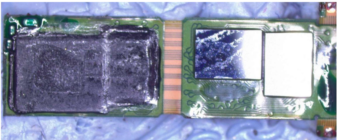
The AM_AU5_KIT312 main PCB module back side
