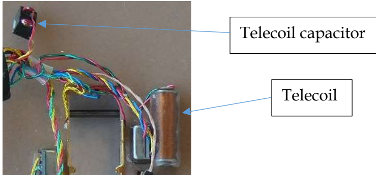
The AM_AU5_KIT312 telecoil mount (Optional)
