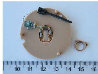
Kit312 radio module faceplate
