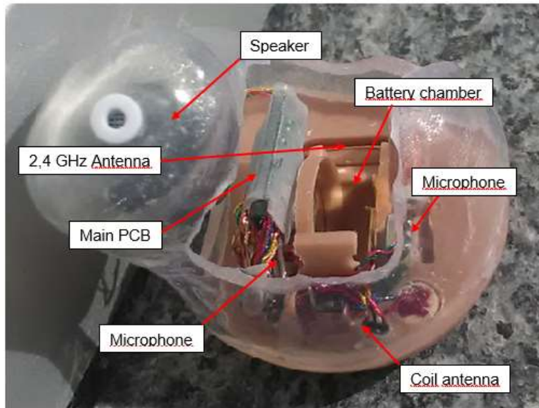
Aurora5 Kit312 Radio Model – 3D overview
