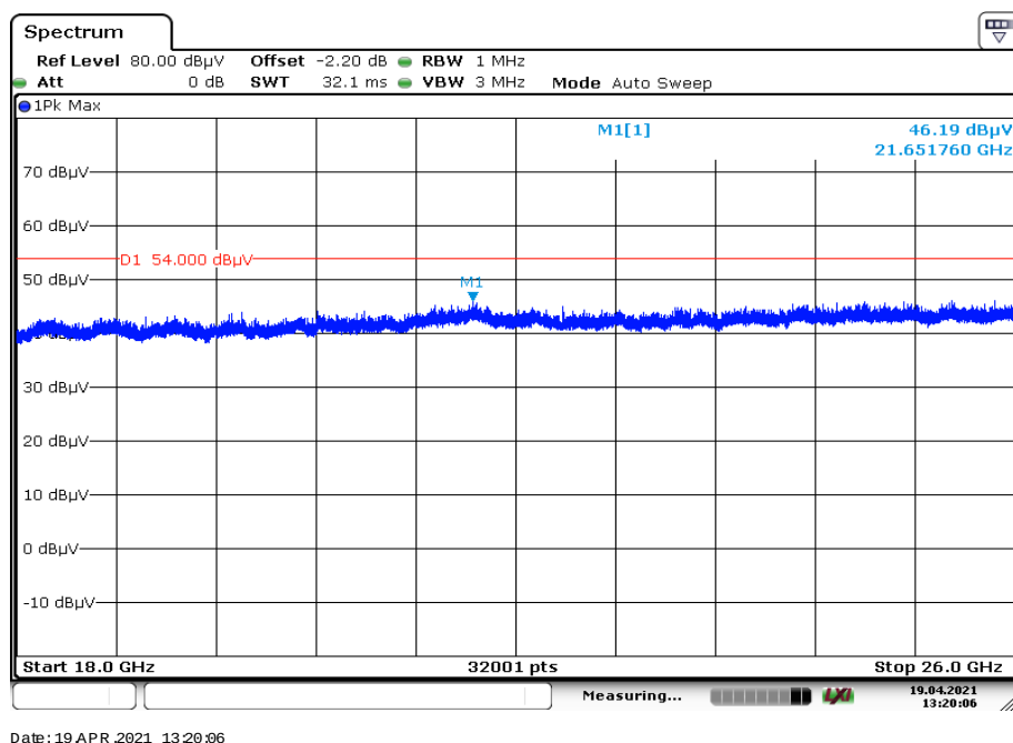
Plot 14: 18 GHz to 26 GHz, TX mode, 2478 MHz, vertical & horizontal polarization, 2 Msps
