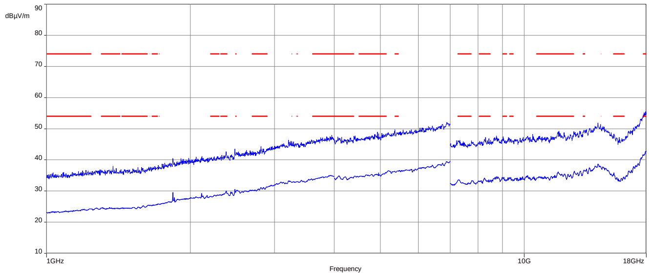
Plot 13: 1 GHz to 18 GHz, TX mode, 2478 MHz, vertical & horizontal polarization, 2 Msps
