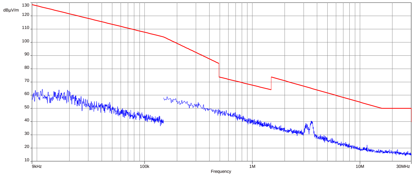
Plot 7: 9 kHz to 30 MHz, 2478 MHz, transmit mode, 2 Msps
