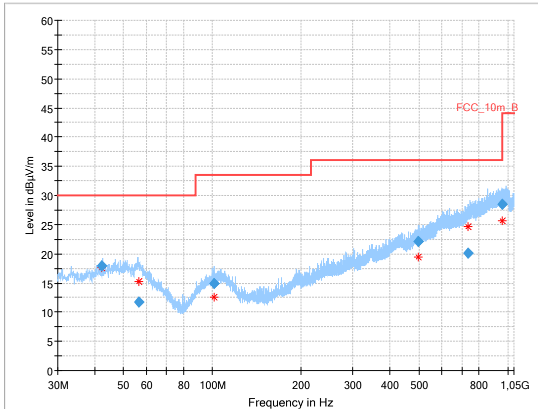
Plot 6: 30 MHz to 1 GHz, TX mode, 2476 MHz, vertical & horizontal polarization, 2 Msps
