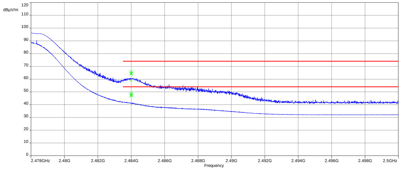
Plot 5: Upper restricted band, 2478 MHz, 2 Msps
