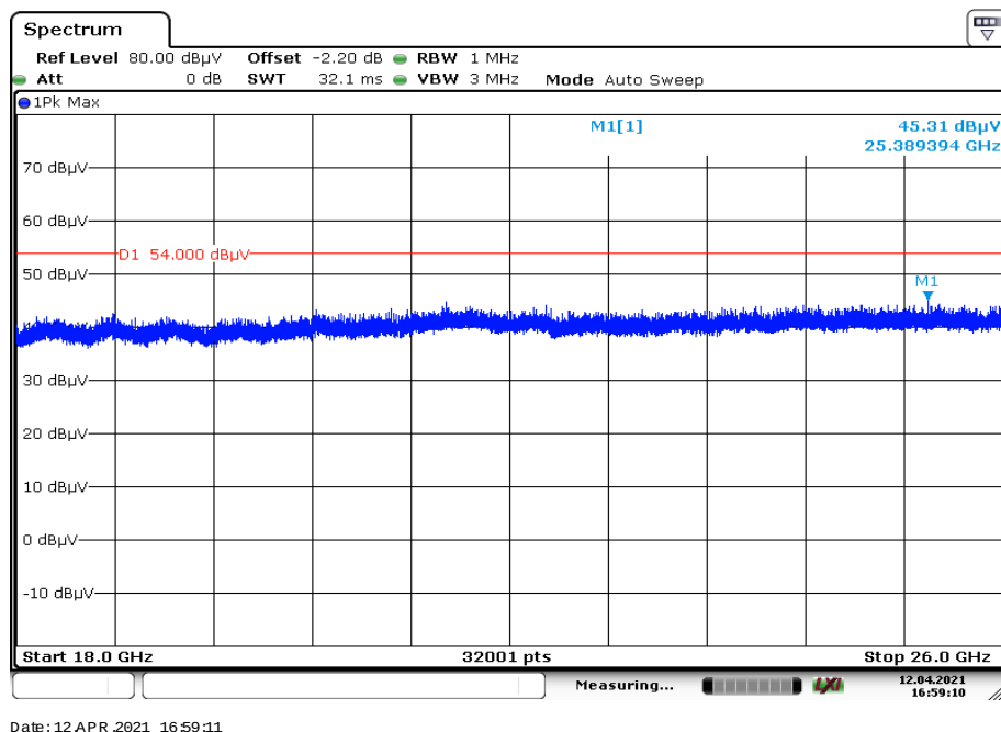
Plot 12: 18 GHz to 26 GHz, TX mode, 2476 MHz, vertical & horizontal polarization, 2 Msps
