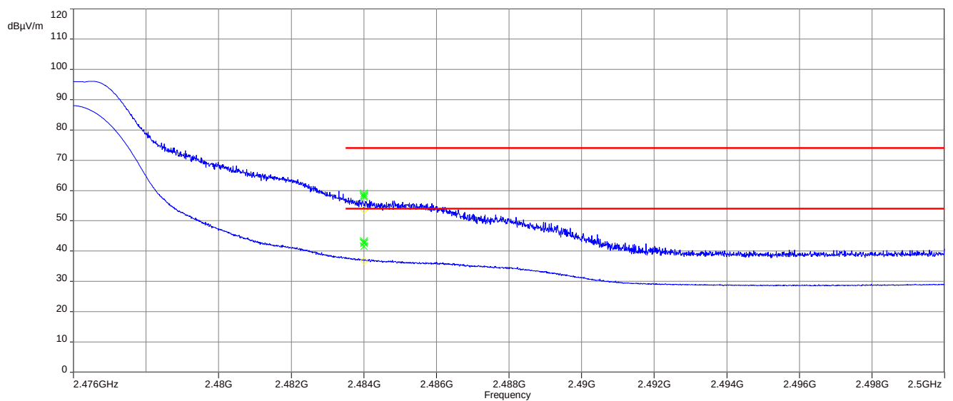
Plot 4: Upper restricted band, 2476 MHz, 2 Msps
