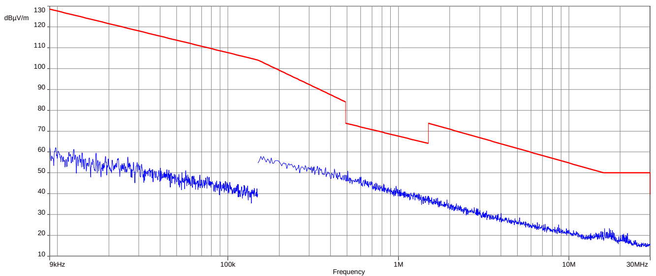
Plot 6: 9 kHz to 30 MHz, 2476 MHz, transmit mode, 2 Msps
