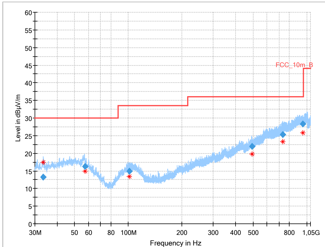
Plot 7: 30 MHz to 1 GHz, TX mode, 2478 MHz, vertical & horizontal polarization, 2 Msps
