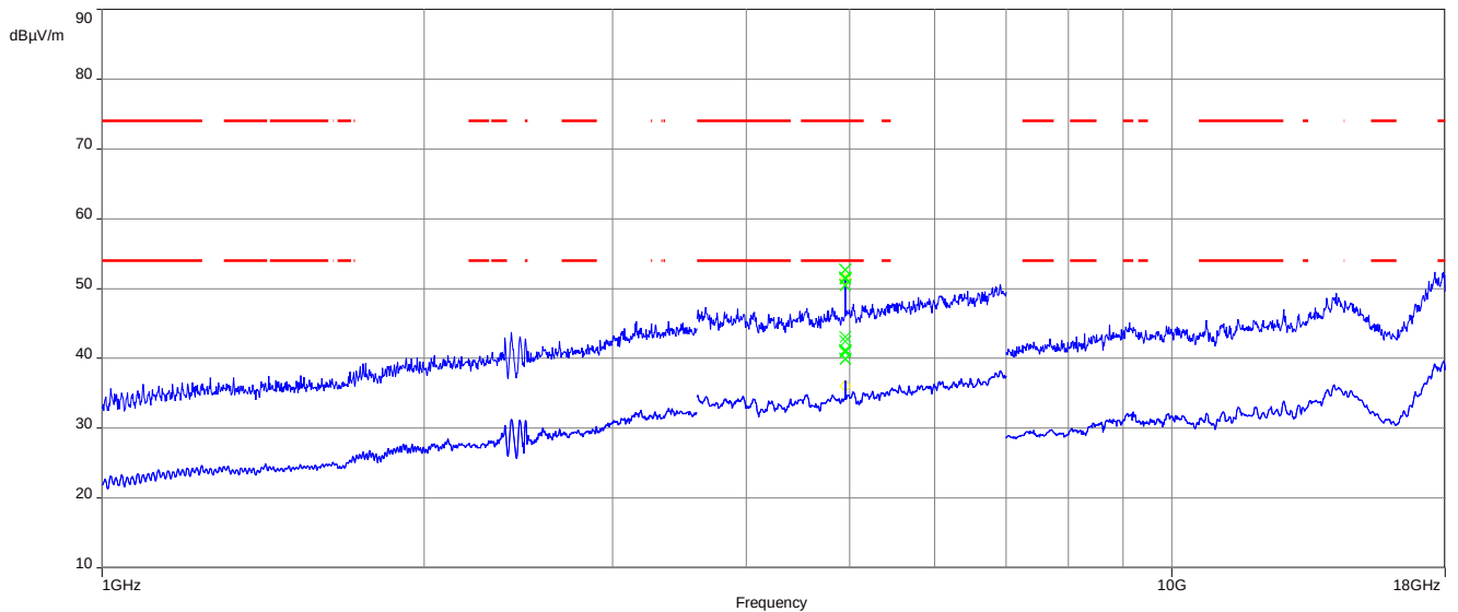
Plot 11: 1 GHz to 18 GHz, TX mode, 2476 MHz, vertical & horizontal polarization, 2 Msps
