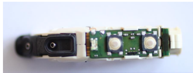
Radio module from the top side (button side)
