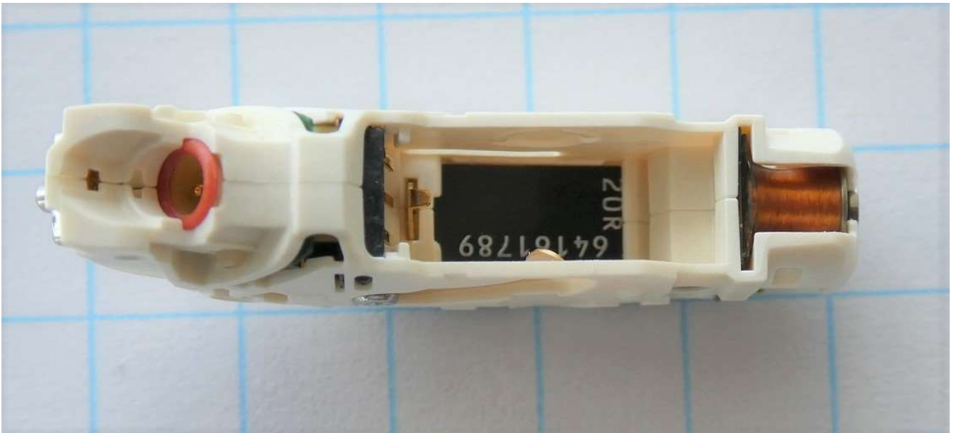
Bottom side with interface connector for speakers/ Bluetooth antenna (left). Telecoil at right.
