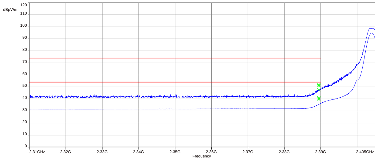
Plot 3: Lower restricted band, 2 Msps
