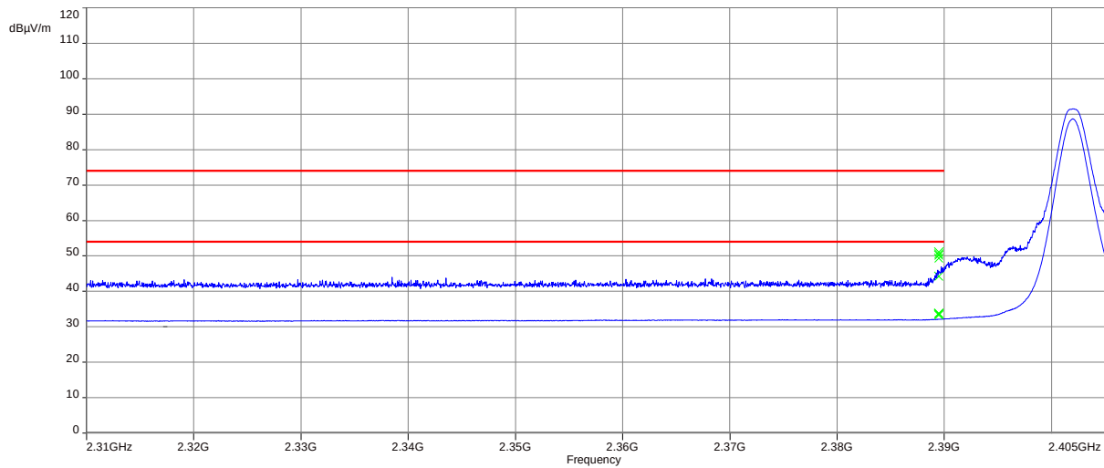
Plot 1: Lower restricted band, 1 Msps
