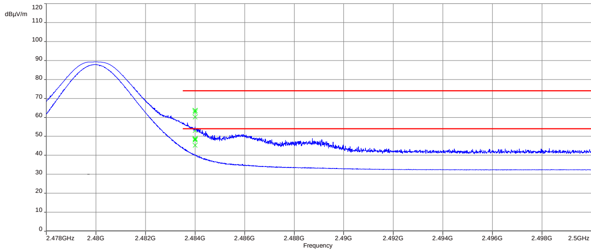
Plot 2: Upper restricted band, 1 Msps
