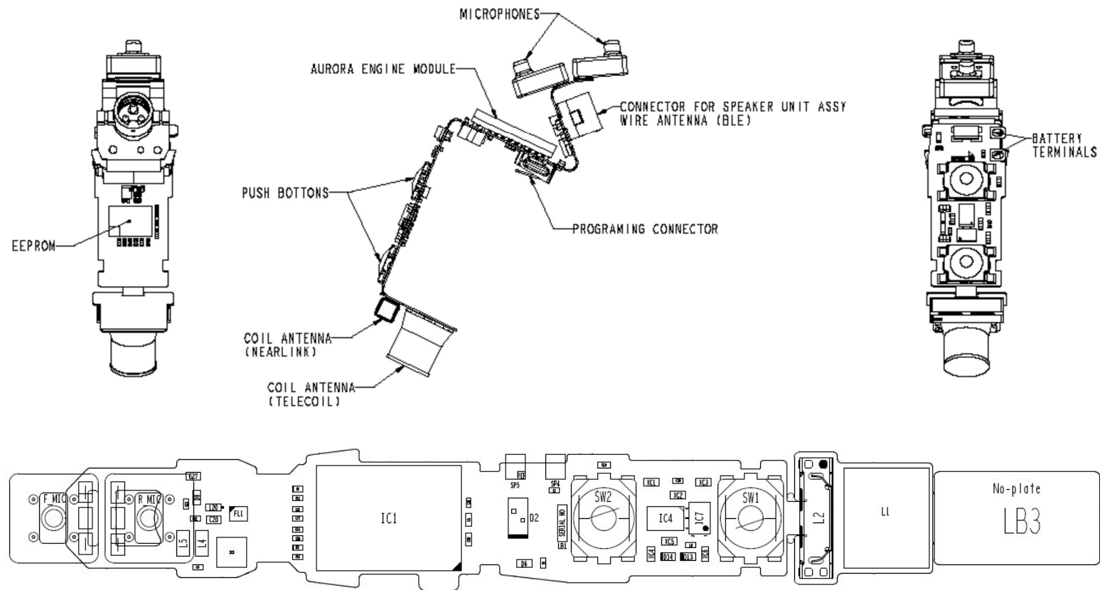
Aurora5 miniRITE T R Radio Model – Main PCB – Top side
