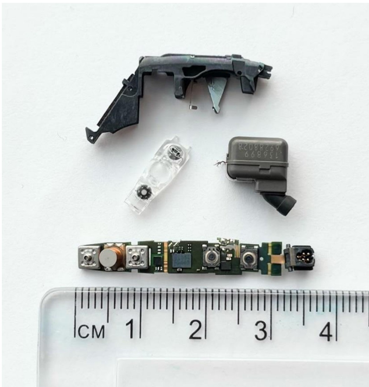
Picture 1 Module parts, rack, microphone gasket, speaker and PCB.
