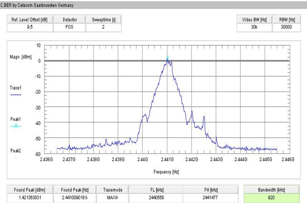
Plot 2: middle channel – 2441 MHz, GFSK modulation
