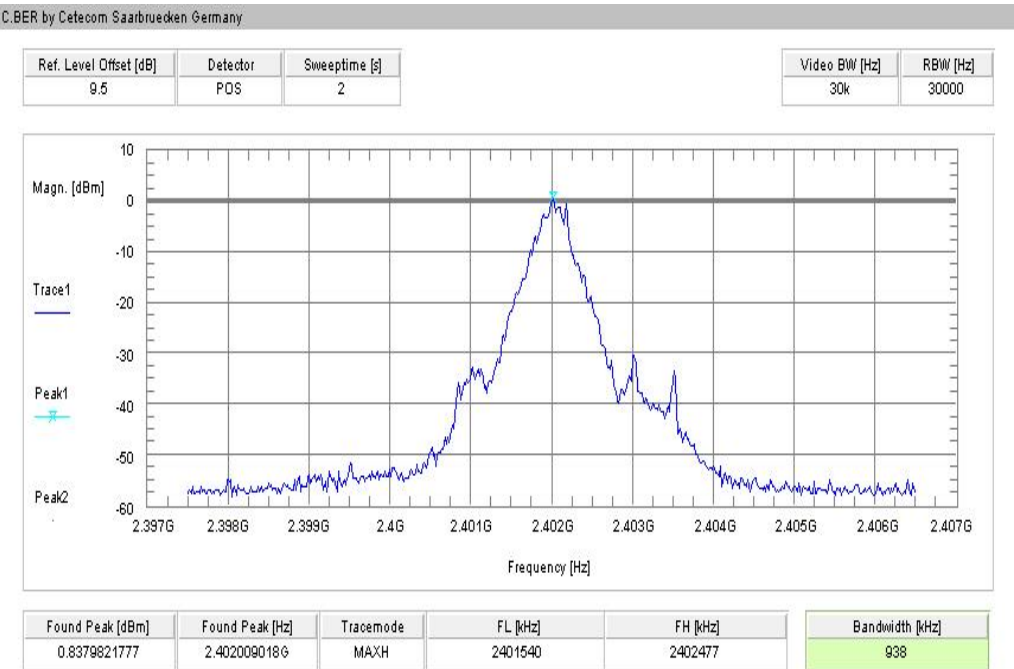
Plot 1: lowest channel – 2402 MHz, GFSK modulation
