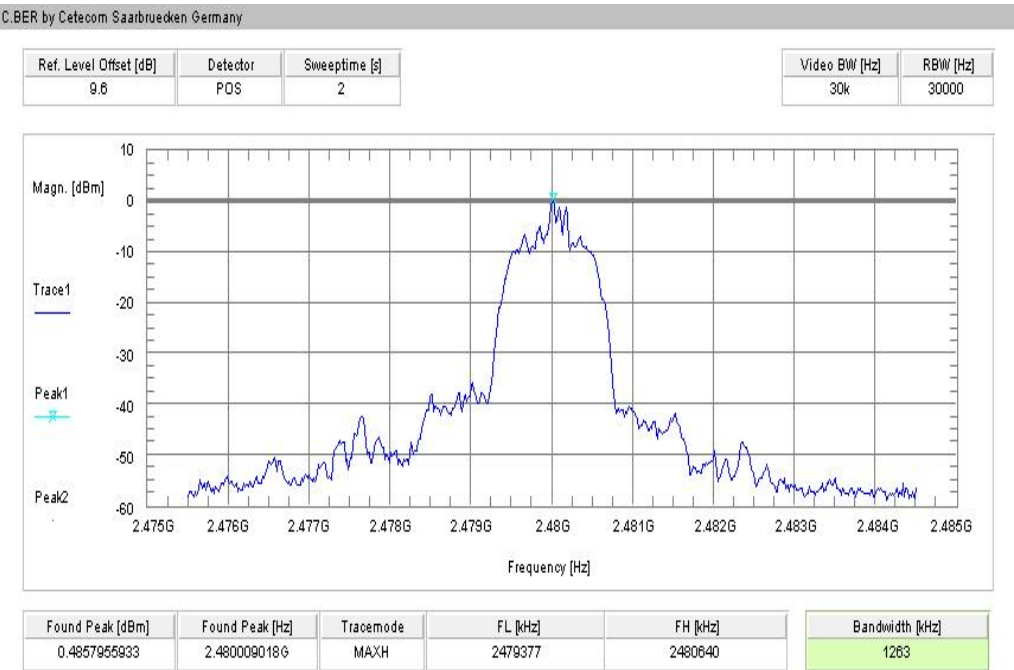
Plot 6: highest channel – 2480 MHz, Pi / DQPSK modulation
