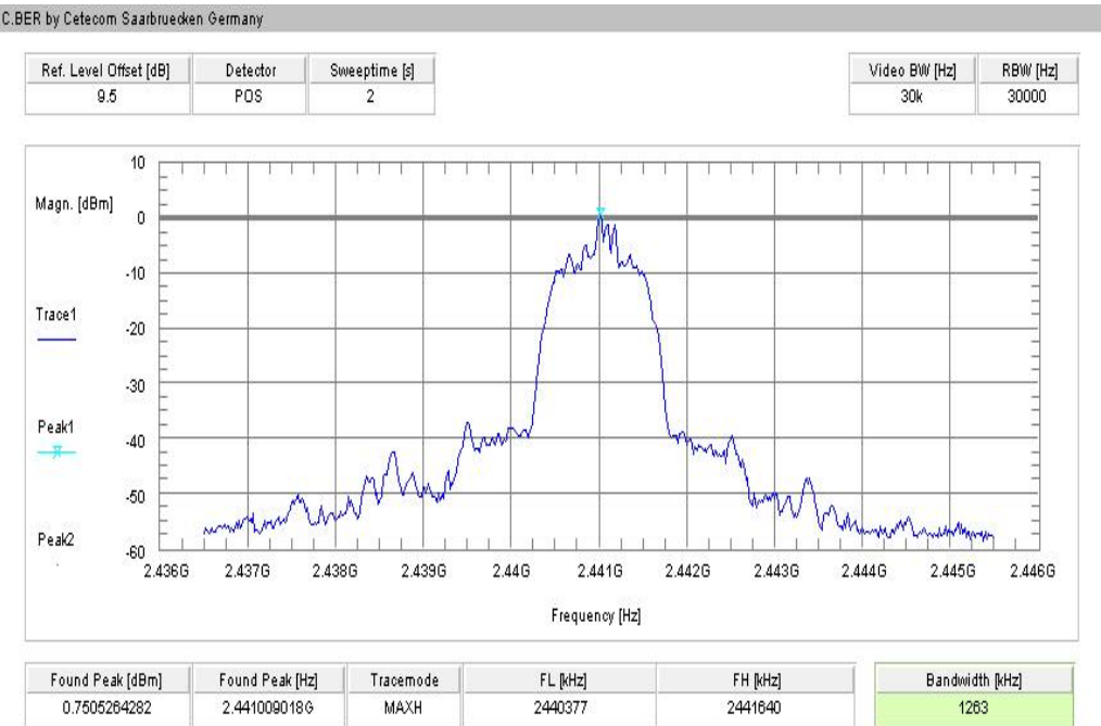
Plot 5: middle channel – 2441 MHz, Pi / DQPSK modulation
