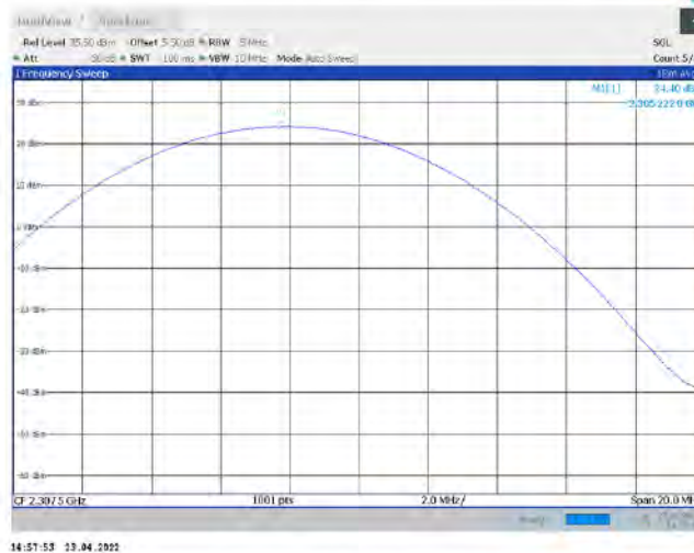
Band30-5MHz-QPSK-27685-1RB#12
