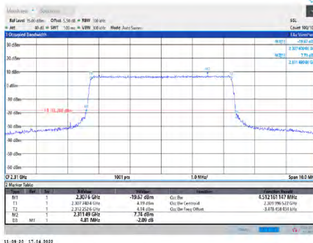
Band30-5MHz-QPSK-27710-25RB#0
