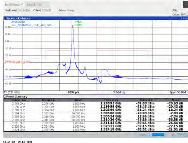
Band30-5MHz-QPSK-27685-25RB#0
