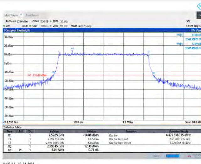
Band38-5MHz-QPSK-38000-25RB#0
