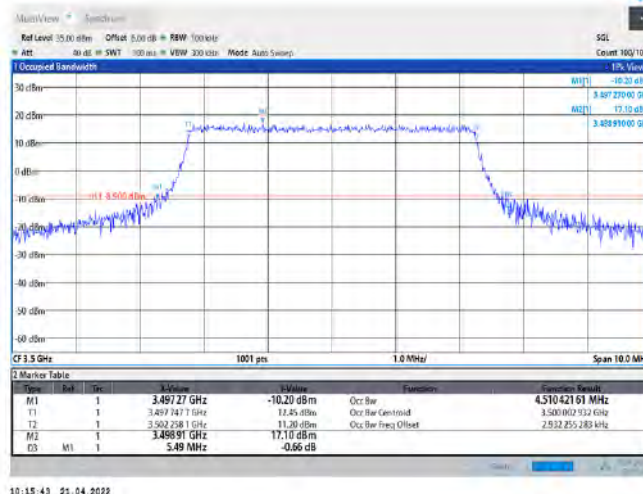
Band42-5MHz-QPSK-42590-25RB#0
