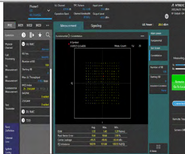
Band42-20MHz-256QAM-42590-100RB#0
