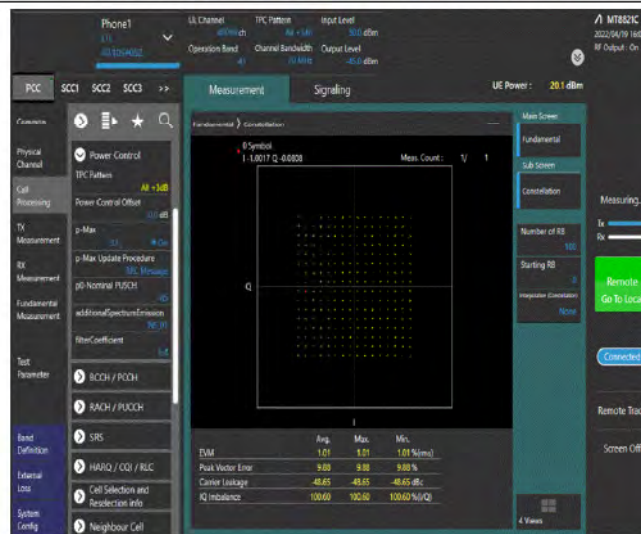
Band43-20MHz-256QAM-45090-100RB#0
