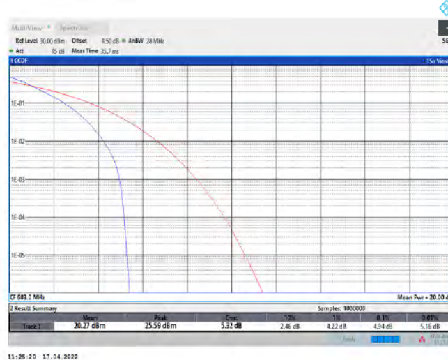
Band71-20MHz-QPSK-133322-100RB#0
