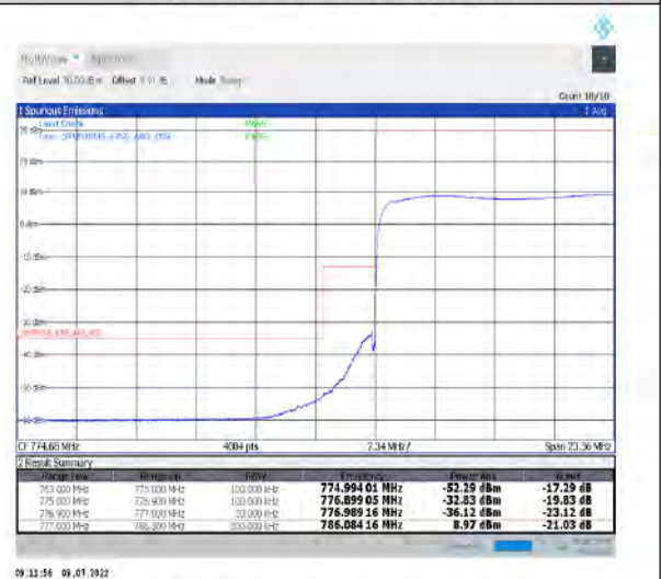
1-N13-PC3-15-10-L-6-CP-QPSK-Outer_Full-52@0-Ant1-PASS-see graph
