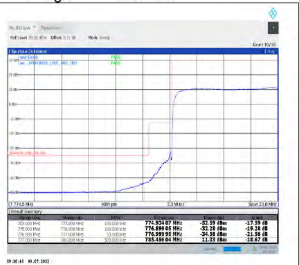
1-N13-PC3-15-10-L-3-DFT-PI2BPSK-Outer_Full-50@0-Ant1-PASS-see graph
