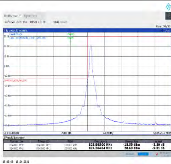
1-N5--15-10-L-1-DFT-PI2BPSK-Edge_1RB_Left-1@0-Ant1-seegraph-PASS-see graph
