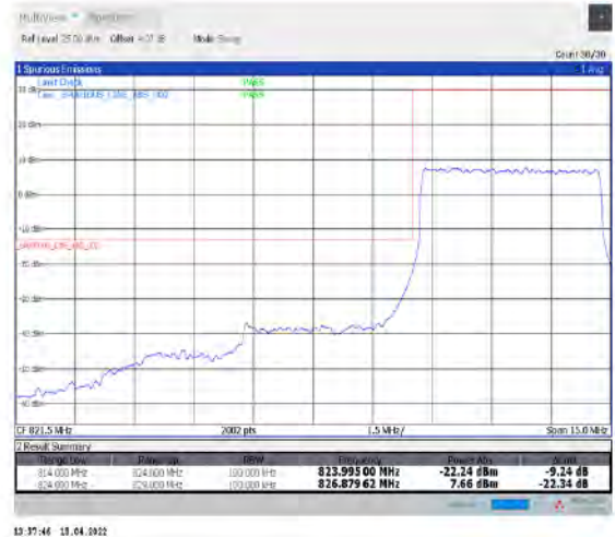
1-N5--15-5-L-3-DFT-PI2BPSK-Outer_Full-25@0-Ant1-seegraph-PASS-see graph
