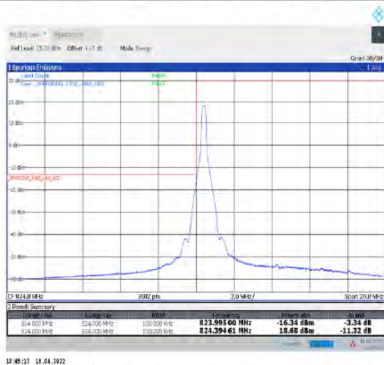
1-N5--15-10-L-4-CP-QPSK-Edge_1RB_Left-1@0-Ant1-seegraph-PASS-see graph
