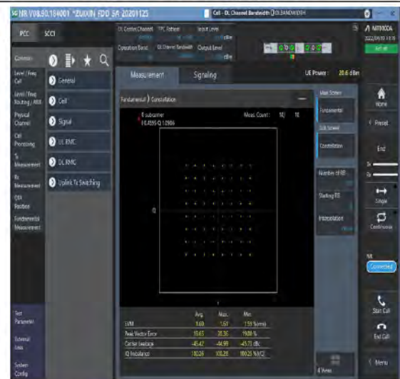
1-N66-PC3-15-20-M-4-DFT-64QAM-Outter_Full-100@0-Ant1-see graph-PASS
