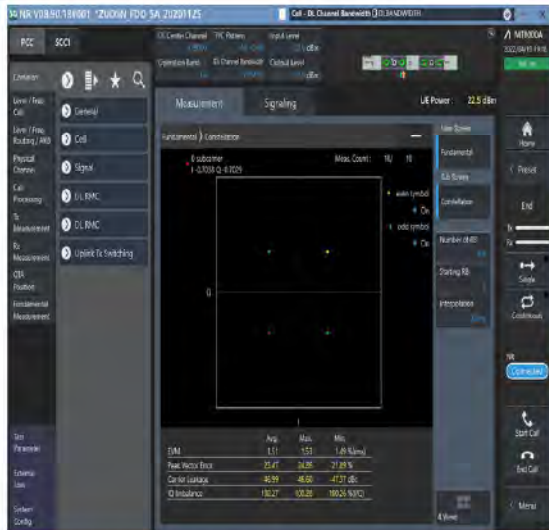
1-N66-PC3-15-20-M-1-DFT-PI2BPSK-Outter_Full-100@0-Ant1-see graph-PASS
