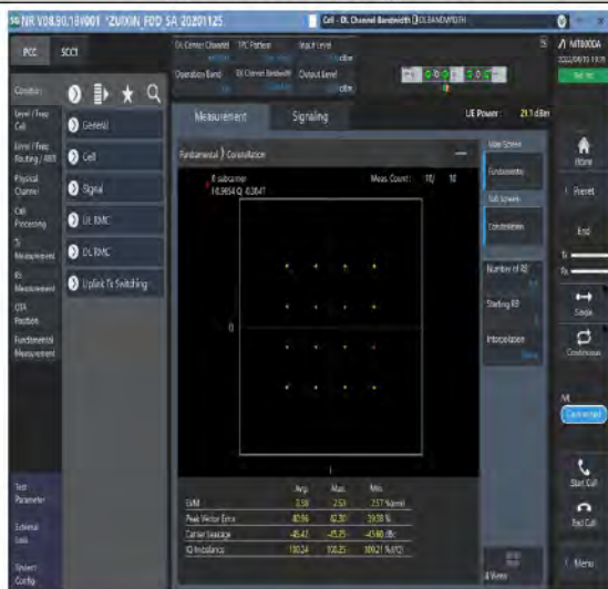
1-N66-PC3-15-20-M-3-DFT-16QAM-Outter_Full-100@0-Ant1-see graph-PASS
