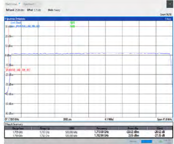
1-N66-PC3-15-40-L-3-DFT-PI2BPSK-Outer_Full-216@0-Ant1-seegraph-PASS-see graph
