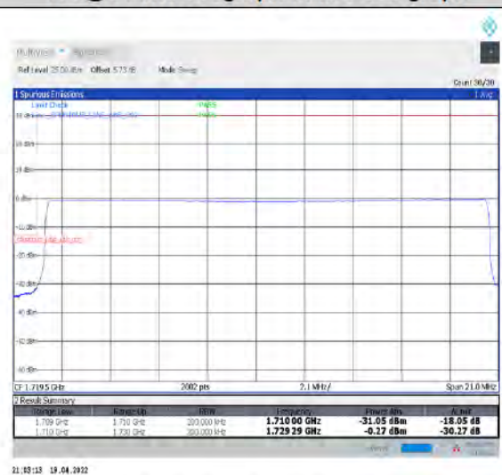
1-N66-PC3-15-20-L-6-CP-QPSK-Outer_Full-106@0-Ant1-seegraph-PASS-see graph
