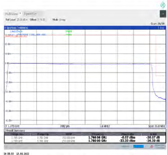
1-N66-PC3-15-15-H-6-CP-QPSK-Outer_Full-79@0-Ant1-seegraph-PASS-see graph
