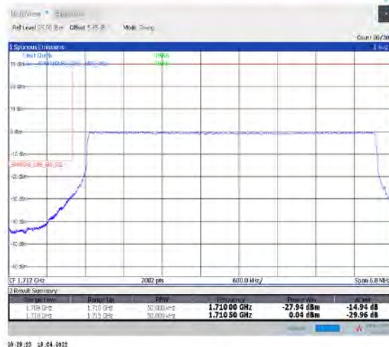
1-N66-PC3-15-5-L-6-CP-QPSK-Outer_Full-25@0-Ant1-seegraph-PASS-see graph
