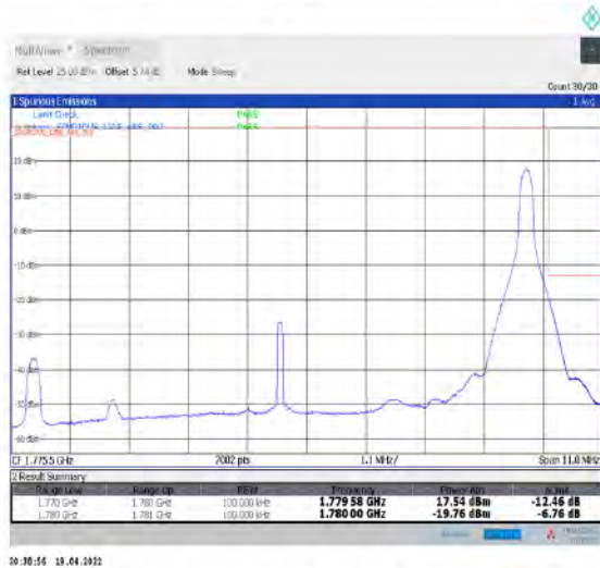
1-N66-PC3-15-10-H-5-CP-QPSK-Edge_1RB_Right-1@51-Ant1-seegraph-PASS-see graph
