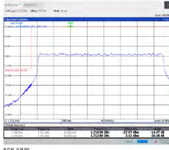
1-N66-PC3-15-5-L-3-DFT-PI2BPSK-Outer_Full-25@0-Ant1-seegraph-PASS-see graph
