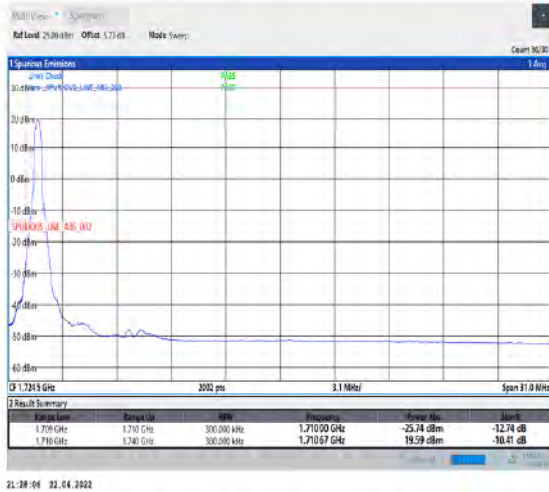
1-N66-PC3-15-30-L-4-CP-QPSK-Edge_1RB_Left_1@0-Ant1-seegraph-PASS-see graph
