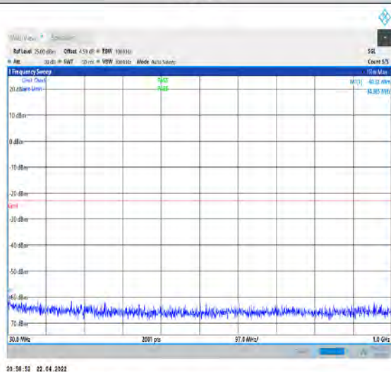
1-N66-PC3-15-40-L-1-DFT-PI2BPSK- Inner_1RB_Left-1@1-30-1000-Ant1--60.92--23- PASS
