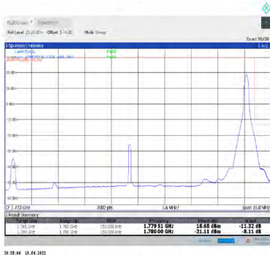
1-N66-PC3-15-15-H-5-CP-QPSK-Edge_1RB_Right-1@78-Ant1-seegraph-PASS-see graph
