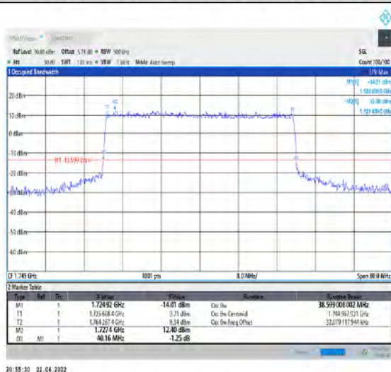
1-N66-PC3-15-40-M-7-CP-16QAM-Outer_Full-216@0-Ant1-38.599-40.160-≤40-PASS
