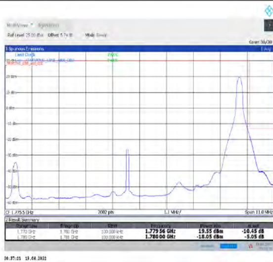
1-N66-PC3-15-10-H-2-DFT-PI2BPSK-Edge_1RB_Right-1@51-Ant1-seegraph-PASS-see graph
