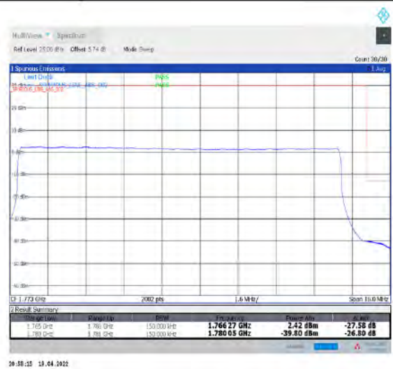
1-N66-PC3-15-15-H-3-DFT-PI2BPSK-Outer_Full-75@0-Ant1-seegraph-PASS-see graph
