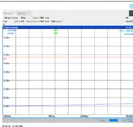
1-N66-PC3-15-40-L-1-DFT-PI2BPSK- Inner_1RB_Left-1@1-0.15-30-Ant1--86.88--33-PASS
