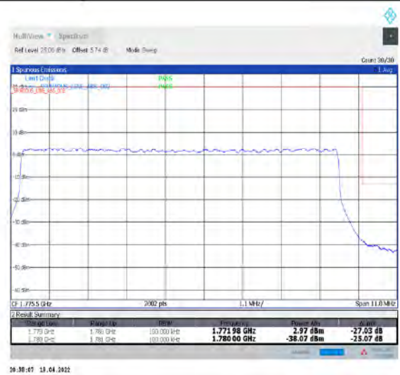
1-N66-PC3-15-10-H-3-DFT-PI2BPSK-Outer_Full-50@0-Ant1-seegraph-PASS-see graph
