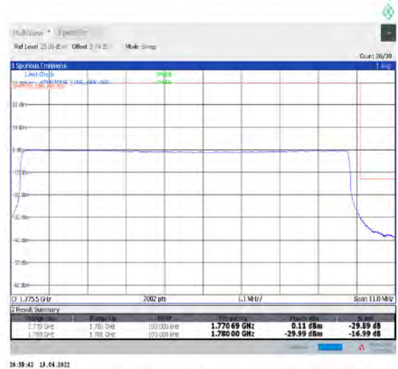
1-N66-PC3-15-10-H-6-CP-QPSK-Outer_Full-52@0-Ant1-seegraph-PASS-see graph
