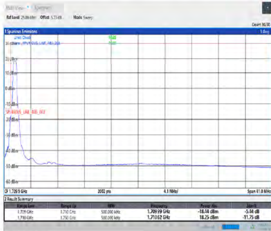
1-N66-PC3-15-40-L-4-CP-QPSK-Edge_1RB_Left-1@0-Ant1-seegraph-PASS-see graph
