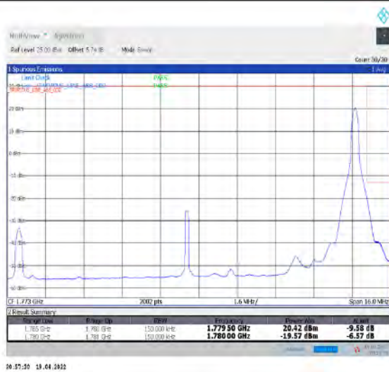
1-N66-PC3-15-15-H-2-DFT-PI2BPSK-Edge_1RB_Right-1@78-Ant1-seegraph-PASS-see graph
