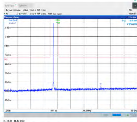
1-N66-PC3-15-40-H-1-DFT-PI2BPSK- Inner_1RB_Left-1@1-1000-3000-Ant1--45.49--13- PASS
