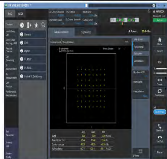
1-N70-PC3-15-15-M-8-CP-64QAM-Outer_Full-79@0-Ant1-see graph-PASS
