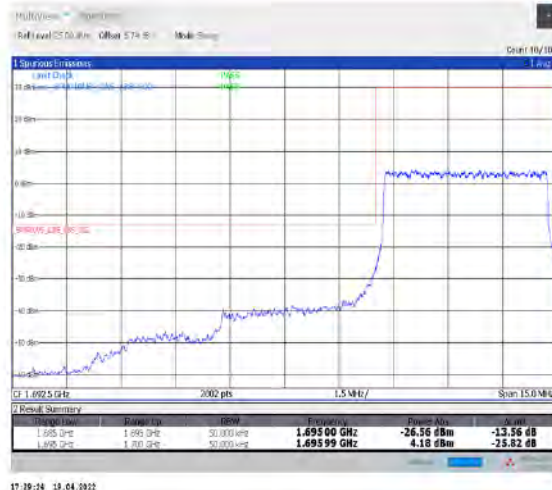
1-N70--15-5-L-3-DFT-PI2BPSK-Outer_Full-25@0-Ant1-seegraph-PASS-see graph
