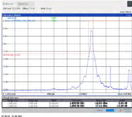
1-N70--15-5-L-1-DFT-PI2BPSK-Edge_1RB_Left-1@0-Ant1-seegraph-PASS-see graph
