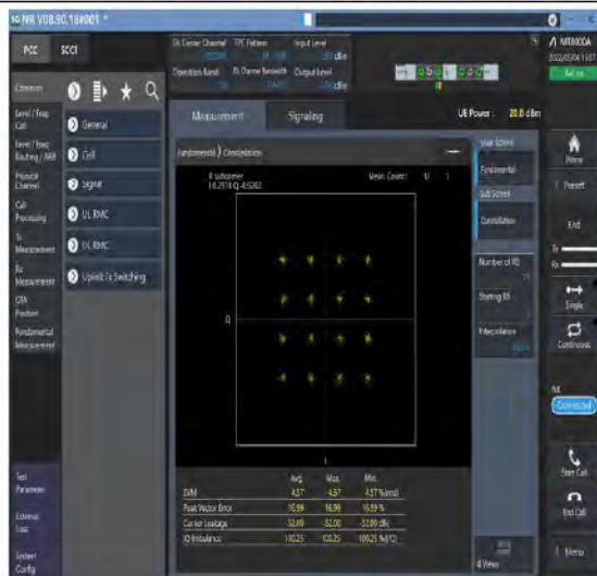
1-N70-PC3-15-15-M-7-CP-16QAM-Outer_Full-79@0-Ant1-see graph-PASS
