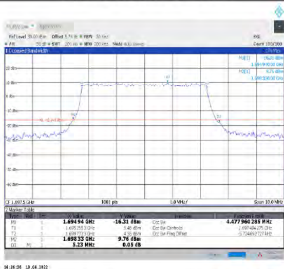
1-N70-15-5-L-7-CP-16QAM-Outer_Full-25@0-Ant1- 4.478-5.230-≤5-PASS
