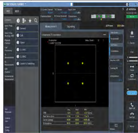
1-N70-PC3-15-15-M-6-CP-QPSK-Outer_Full-79@0-Ant1-see graph-PASS
