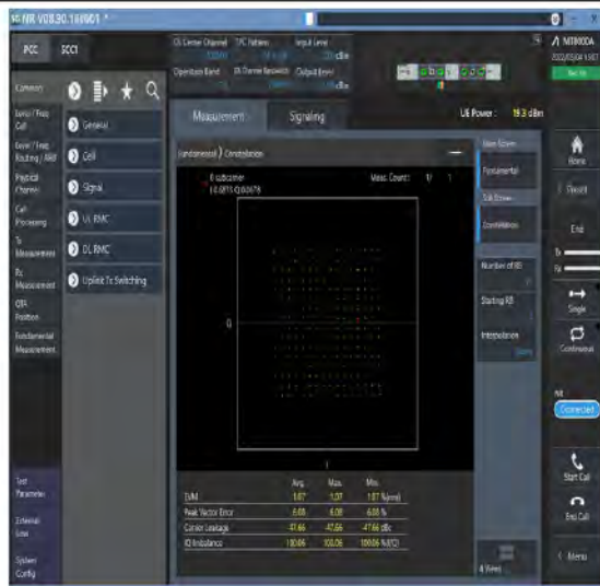
1-N70-PC3-15-15-M-5-DFT-256QAM-Outer_Full-75@0-Ant1-see graph-PASS
