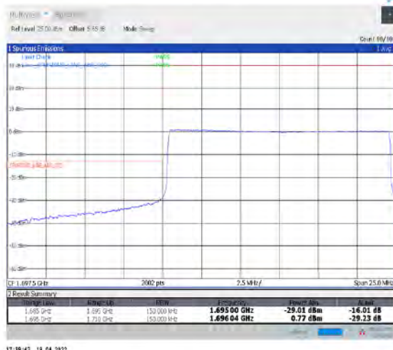
1-N70--15-15-L-6-CP-QPSK-Outer_Full-79@0-Ant1-seegraph-PASS-see graph
