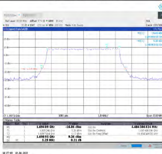
1-N70-15-5-L-8-CP-64QAM-Outer_Full-25@0-Ant1- 4.484-5.250-≤5-PASS
