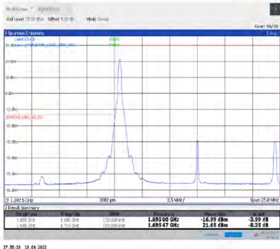
1-N70--15-15-L-1-DFT-PI2BPSK-Edge_1RB_Left-1@0-Ant1-seegraph-PASS-see graph
