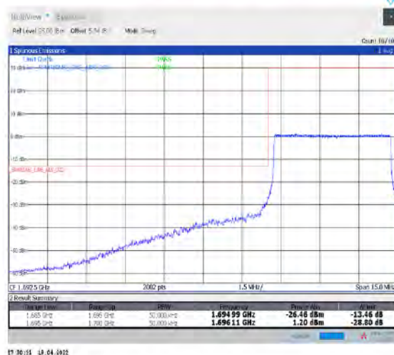
1-N70--15-5-L-6-CP-QPSK-Outer_Full-25@0-Ant1-seegraph-PASS-see graph
