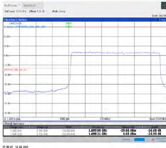
1-N70--15-15-L-3-DFT-PI2BPSK-Outer_Full-75@0-Ant1-seegraph-PASS-see graph
