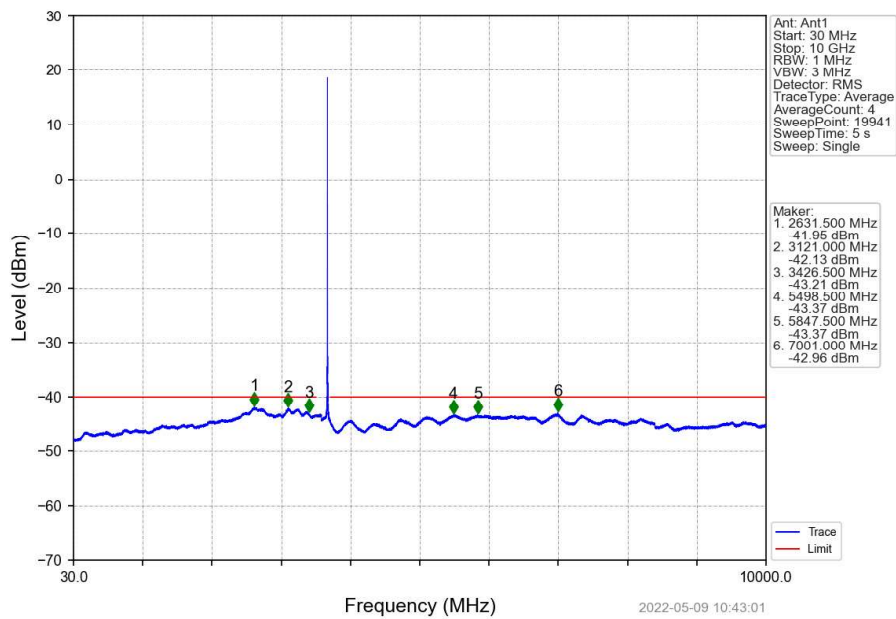
Band48_15MHz_16QAM_HCH_3692.5MHz_RB_1_0_NTNV
