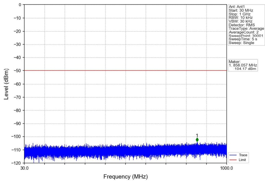
n48_30kHz_SISO_NTNV_10MHz_CP-OFDM QPSK_3624.99MHz_Edge_1RB_Left
