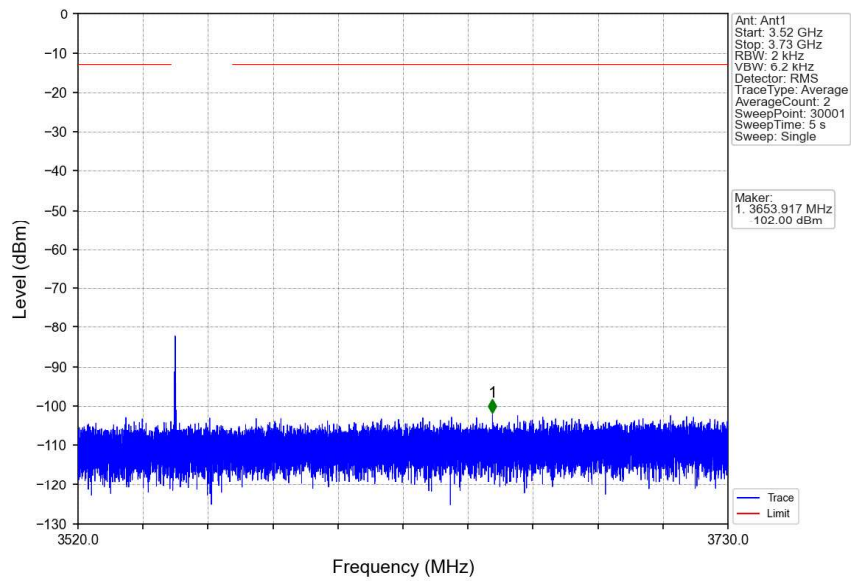
n48_30kHz_SISO_NTNV_20MHz_DFT-s-OFDM QPSK_3624.99MHz_Edge_1RB_Left
