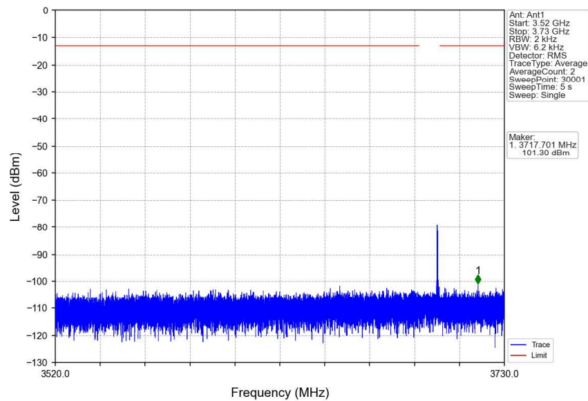
n48_30kHz_SISO_NTNV_10MHz_CP-OFDM QPSK_3694.98MHz_Inner_1RB_Right
