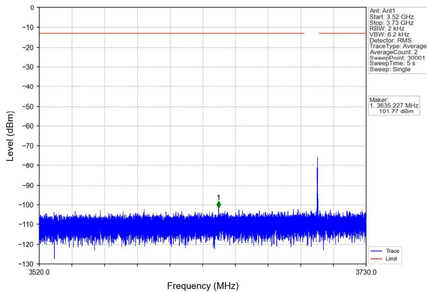
n48_30kHz_SISO_NTNV_10MHz_DFT-s-OFDM QPSK_3694.98MHz_Inner_1RB_Right
