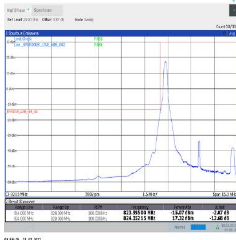
1-N5-15-5-L-4-CP-QPSK-Edge_1RB_Left-1@0-Ant1-seegraph-PASS-see graph
