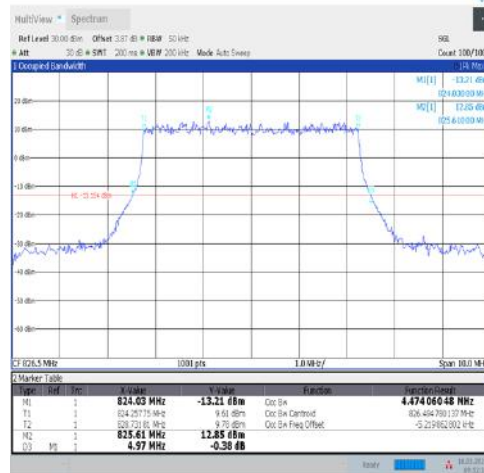
1-N5-15-5-L-2-DFT-PI2BPSK-Outer_Full-25@0-Ant1- 4.474-4.970-≤5-PASS
