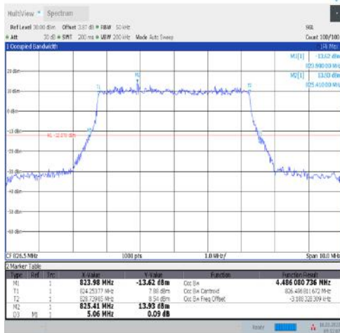
1-N5-15-5-L-1-DFT-QPSK-Outer_Full-25@0-Ant1- 4.486-5.060-≤5-PASS
