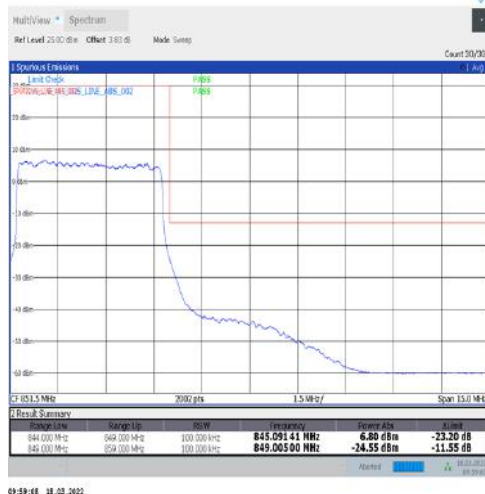
1-N5-15-5-H-3-DFT-PI2BPSK-Outer_Full-25@0-Ant1-seegraph-PASS-see graph
