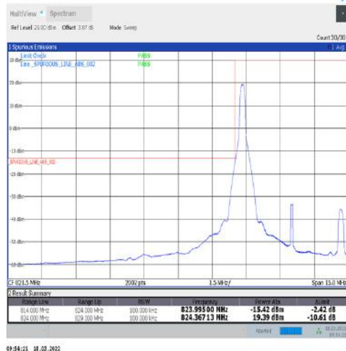
1-N5-15-5-L-1-DFT-PI2BPSK-Edge_1RB_Left-1@0-Ant1-seegraph-PASS-see graph
