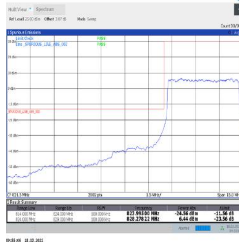
1-N5-15-5-L-3-DFT-PI2BPSK-Outer_Full-25@0-Ant1-seegraph-PASS-see graph
