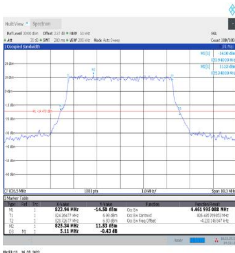
1-N5-15-5-L-3-DFT-16QAM-Outer_Full-25@0-Ant1- 4.462-5.110-≤5-PASS
