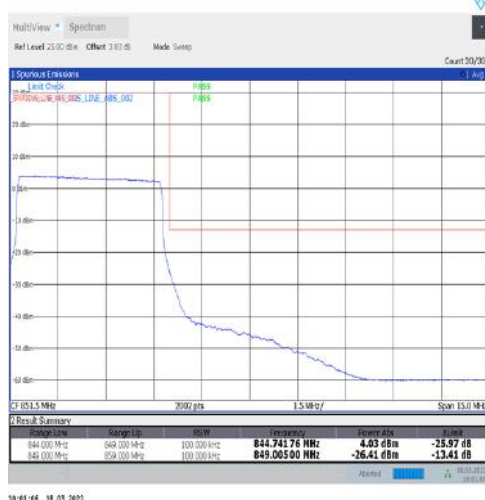
1-N5-15-5-H-6-CP-QPSK-Outer_Full-25@0-Ant1-seegraph-PASS-see graph
