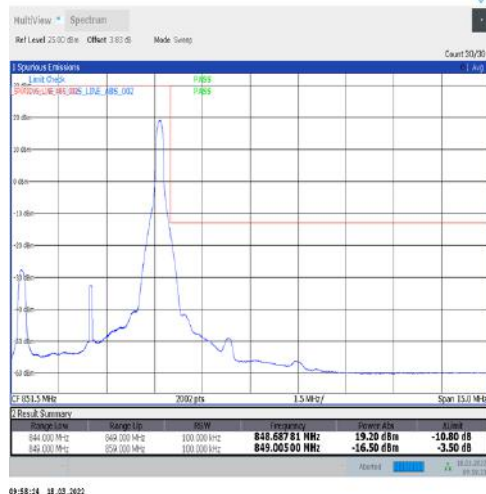
1-N5-15-5-H-2-DFT-PI2BPSK-Edge_1RB_Right-1@24-Ant1-seegraph-PASS-see graph
