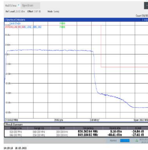
1-N5-15-20-H-3-DFT-PI2BPSK-Outer_Full-100@0-Ant1-seegraph-PASS-see graph
