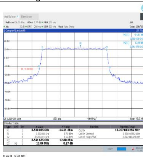
1-N77-3450-3550-30-20-H-6-CP-QPSK-Outer_Full-51@0-Ant1-18.207-19.840-≤20-PASS
