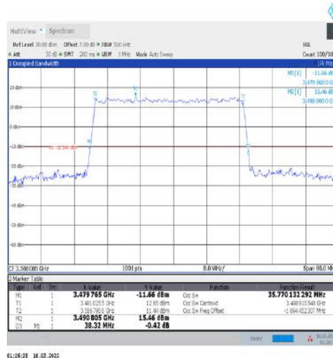
1-N77-3450-3550-30-40-M-3-DFT-16QAM-Outer_Full-100@0-Ant1-35.77-38.320-≤40-PASS
