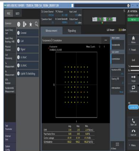
1-N77-3450-3550-30-100-M-8-CP-64QAM-Outer_Full-273@0-Ant1-see graph-PASS
