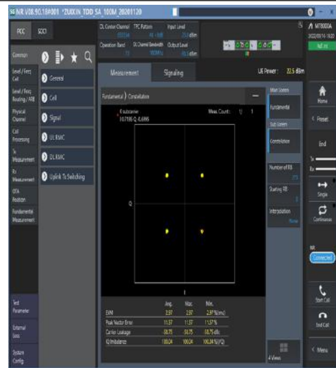
1-N77-3450-3550-30-100-M-6-CP-QPSK-Outer_Full-273@0-Ant1-see graph-PASS
