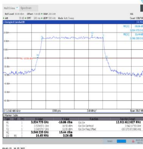
1-N77-3450-3550-30-15-H-3-DFT-16QAM-Outer_Full-36@0-Ant1-12.922-14.490-≤15-PASS
