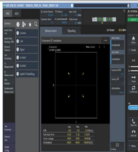
1-N77-3450-3550-30-100-M-2-DFT-QPSK- Outer_Full-270@0-Ant1-see graph-PASS
