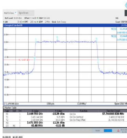
1-N77-3450-3550-30-60-L-6-CP-QPSK-Outer_Full-162@0-Ant1-57.745-60.480-≤60-PASS
