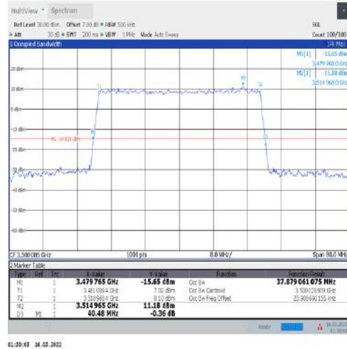
1-N77-3450-3550-30-40-M-9-CP-256QAM-Outer_Full-106@0-Ant1-37.879-40.480-≤40-PASS
