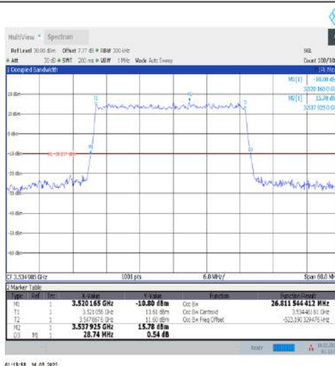
1-N77-3450-3550-30-30-H-1-DFT-QPSK-Outer_Full-75@0-Ant1-26.812-28.740-≤30-PASS
