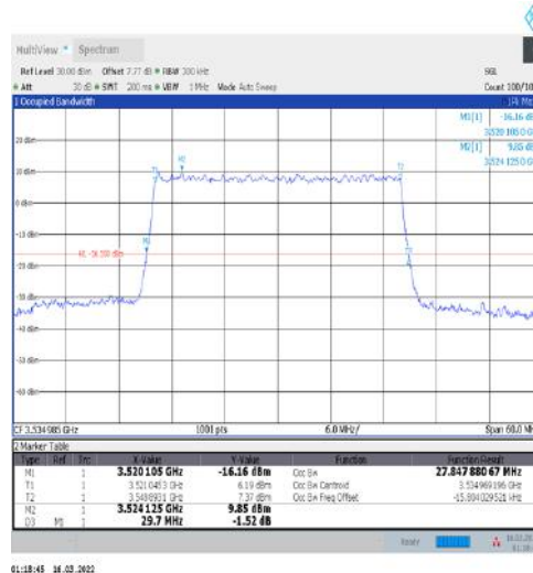
1-N77-3450-3550-30-30-H-9-CP-256QAM-Outer_Full-78@0-Ant1-27.848-29.700-≤30-PASS
