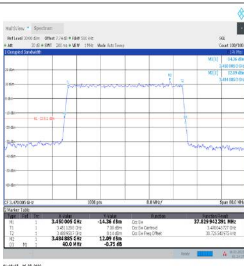
1-N77-3450-3550-30-40-L-9-CP-256QAM-Outer_Full-106@0-Ant1-37.83-40.000-≤40-PASS
