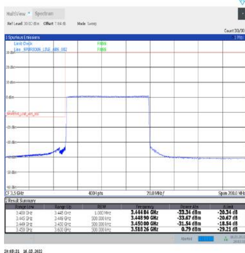
1-N77-3450-3550-30-70-L-6-CP-QPSK-Outer_Full-189@0-Ant1-PASS-see graph
