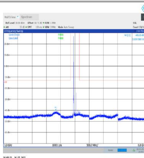
1-N77-3450-3550-30-100-H-1-DFT-PI2BPSK- Inner_1RB_Left-1@1-1000-6000-Ant1--40.63--13- PASS
