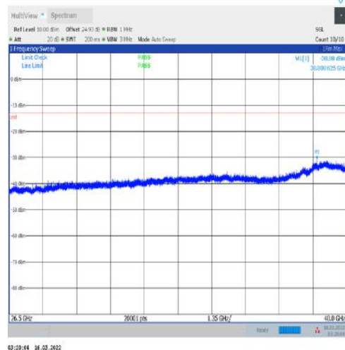
1-N77-3450-3550-30-100-H-1-DFT-PI2BPSK- Inner_1RB_Left-1@1-26500-40000-Ant1--30.98--13- PASS
