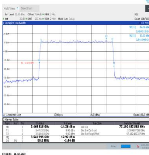
1-N77-3450-3550-30-80-H-5-DFT-256QAM-Outer_Full-216@0-Ant1-77.19-80.800-≤80-PASS
