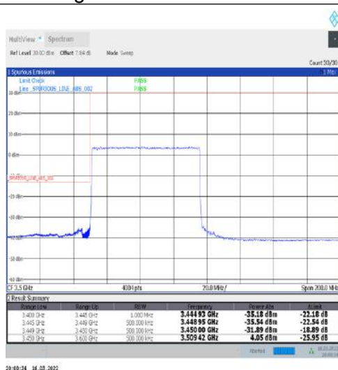
1-N77-3450-3550-30-70-L-3-DFT-PI2BPSK-Outer_Full-180@0-Ant1-PASS-see graph
