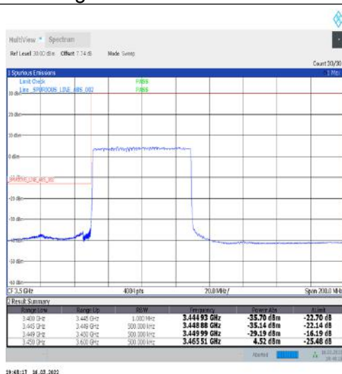
1-N77-3450-3550-30-60-L-3-DFT-PI2BPSK-Outer_Full-162@0-Ant1-PASS-see graph
