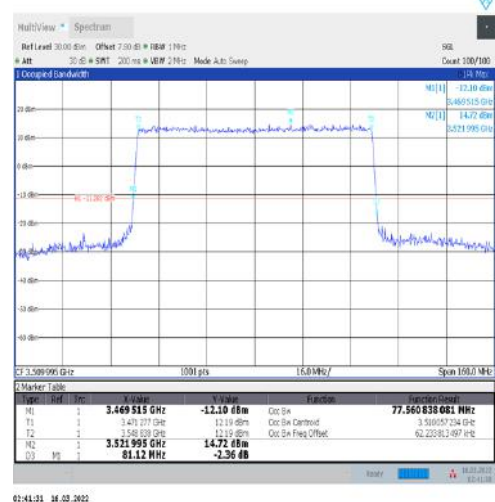
1-N77-3450-3550-30-80-H-6-CP-QPSK-Outer_Full-217@0-Ant1-77.561-81.120-≤80-PASS
