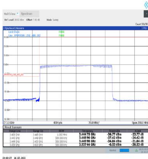
1-N77-3450-3550-30-100-L-6-CP-QPSK-Outer_Full-273@0-Ant1-PASS-see graph
