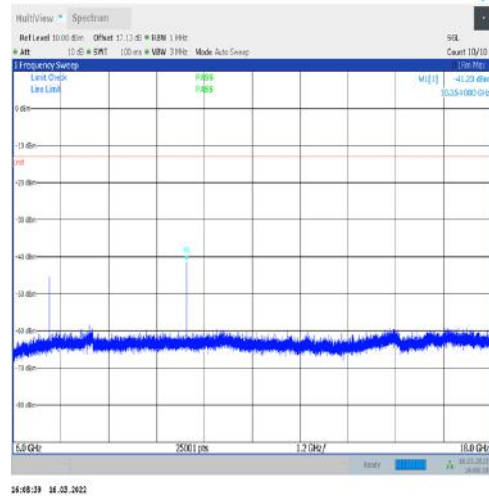
1-N77-3450-3550-30-100-H-1-DFT-PI2BPSK- Inner_1RB_Left-1@1-6000-18000-Ant1--41.23--13- PASS
