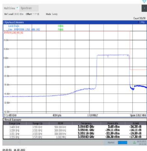
1-N77-3450-3550-30-40-H-6-CP-QPSK-Outer_Full-106@0-Ant1-PASS-see graph
