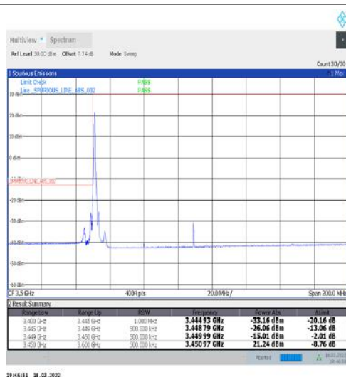
1-N77-3450-3550-30-60-L-1-DFT-PI2BPSK-Edge_1RB_Left-1@0-Ant1-PASS-see graph
