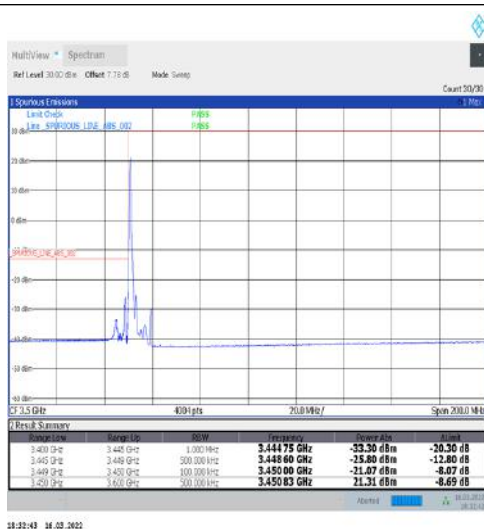
1-N77-3450-3550-30-10-L-1-DFT-PI2BPSK-Edge_1RB_Left-1@0-Ant1-PASS-see graph
