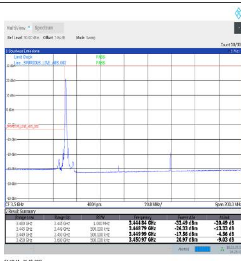
1-N77-3450-3550-30-90-L-1-DFT-PI2BPSK-Edge_1RB_Left-1@0-Ant1-PASS-see graph
