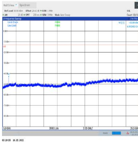
1-N77-3450-3550-30-100-H-1-DFT-PI2BPSK- Inner_1RB_Left-1@1-6000-26500-Ant1--43.88--13- PASS
