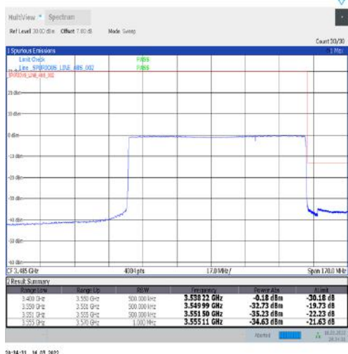
1-N77-3450-3550-30-90-H-6-CP-QPSK-Outer_Full-245@0-Ant1-PASS-see graph
