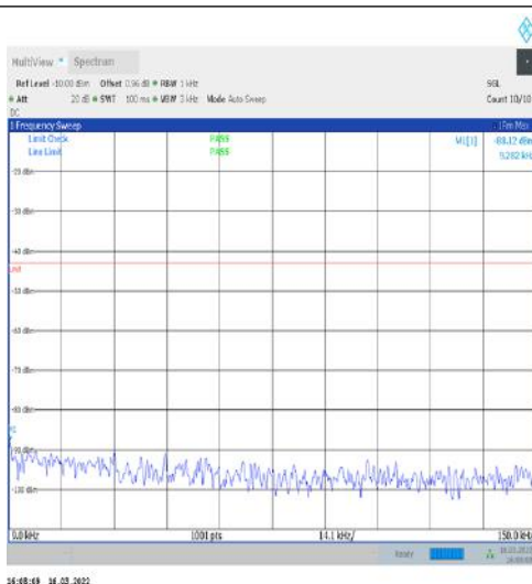
1-N77-3450-3550-30-100-H-1-DFT-PI2BPSK- Inner_1RB_Left-1@1-0.009-0.15-Ant1--88.12--43- PASS
