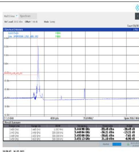
1-N77-3450-3550-30-70-L-1-DFT-PI2BPSK-Edge_1RB_Left-1@0-Ant1-PASS-see graph
