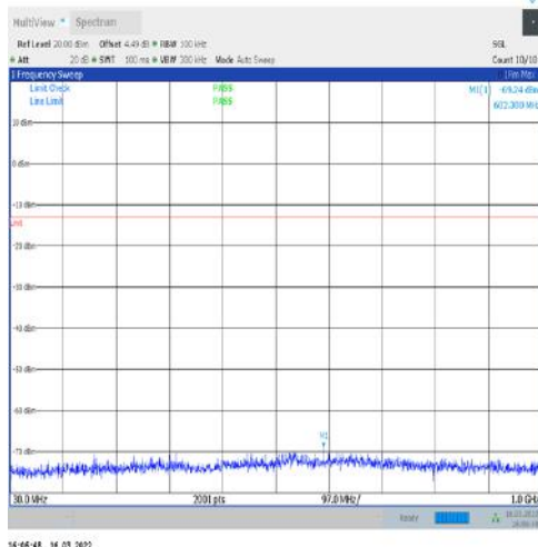
1-N77-3450-3550-30-100-L-1-DFT-PI2BPSK- Inner_1RB_Left-1@1-30-1000-Ant1--69.24--23- PASS
