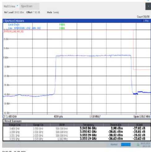
1-N77-3450-3550-30-90-H-3-DFT-PI2BPSK-Outer_Full-240@0-Ant1-PASS-see graph
