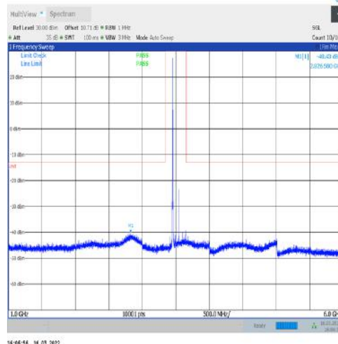
1-N77-3450-3550-30-100-L-1-DFT-PI2BPSK- Inner_1RB_Left-1@1-1000-6000-Ant1--40.43--13- PASS
