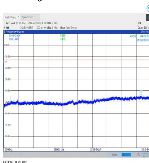
1-N77-3450-3550-30-100-L-1-DFT-PI2BPSK- Inner_1RB_Left-1@1-6000-26500-Ant1--44.28--13- PASS
