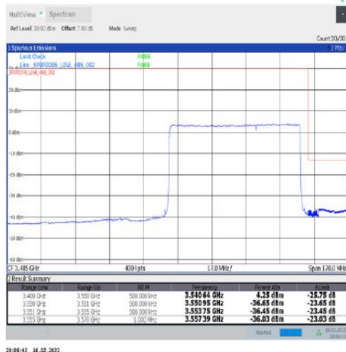
1-N77-3450-3550-30-70-H-3-DFT-PI2BPSK-Outer_Full-180@0-Ant1-PASS-see graph
