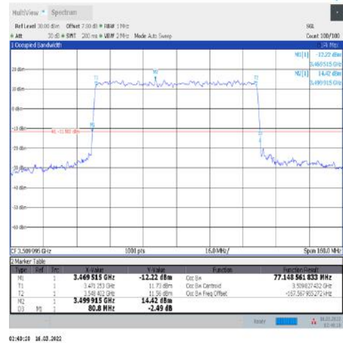
1-N77-3450-3550-30-80-H-4-DFT-64QAM-Outer_Full-216@0-Ant1-77.149-80.800-≤80-PASS
