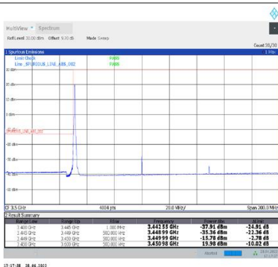
1-N77-3450-3550--30-100-L-4-CP-QPSK-Edge_1RB_Left-1@0-Ant1-PASS-see graph
