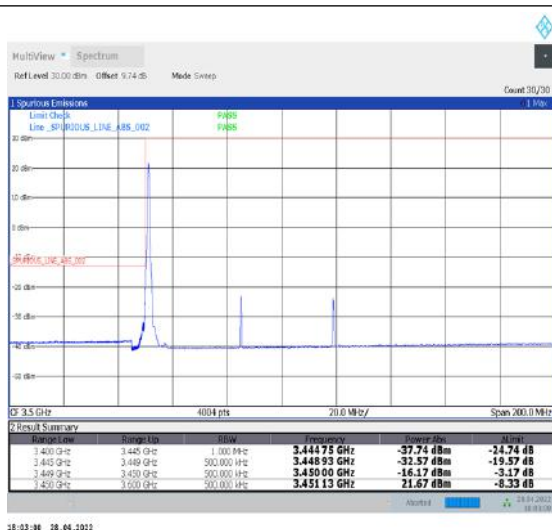
1-N77-3450-3550--30-70-L-4-CP-QPSK-Edge_1RB_Left-1@0-Ant2-PASS-see graph
