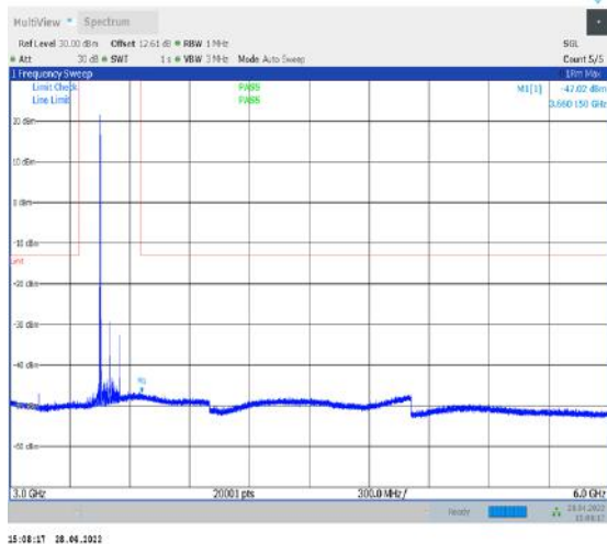
1-N77-3450-3550--30-100-L-1-DFT-QPSK- Edge_1RB_Left-1@0-3000-6000-Ant1--47.02--13- PASS
