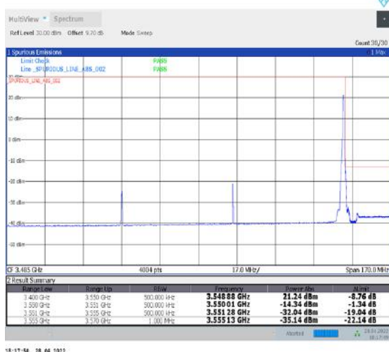
1-N77-3450-3550--30-100-H-5-CP-QPSK-Edge_1RB_Right-1@272-Ant2-PASS-see graph
