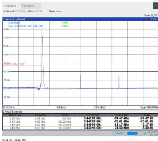
1-N77-3450-3550--30-100-L-4-CP-QPSK-Edge_1RB_Left-1@0-Ant2-PASS-see graph
