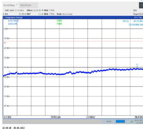
1-N77-3450-3550--30-100-L-1-DFT-QPSK- Edge_1RB_Left-1@0-6000-26000-Ant1--40.24--13- PASS
