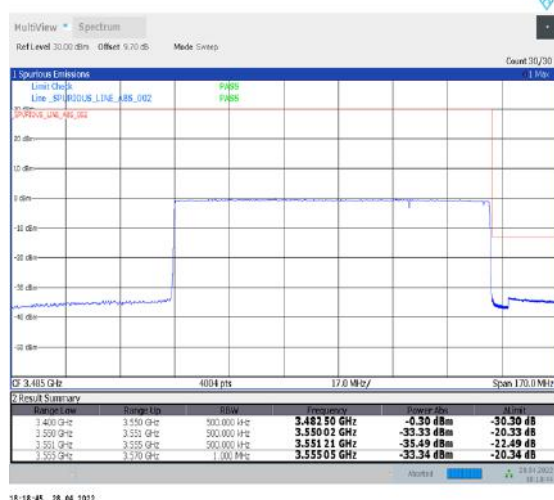
1-N77-3450-3550--30-100-H-6-CP-QPSK-Outer_Full-273@0-Ant2-PASS-see graph
