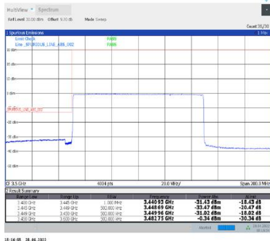
1-N77-3450-3550--30-100-L-6-CP-QPSK-Outer_Full-273@0-Ant2-PASS-see graph
