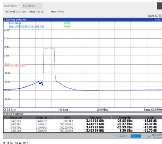
1-N77-3450-3550--30-15-L-6-CP-QPSK-Outer_Full-38@0-Ant2-PASS-see graph
