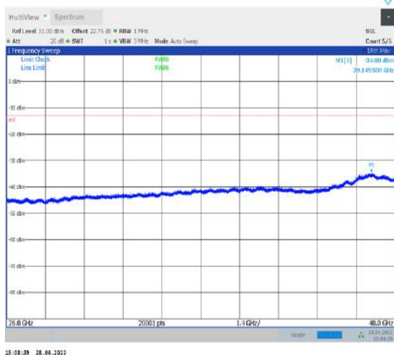
1-N77-3450-3550--30-100-L-1-DFT-QPSK- Edge_1RB_Left-1@0-26000-40000-Ant1--34.80--13- PASS
