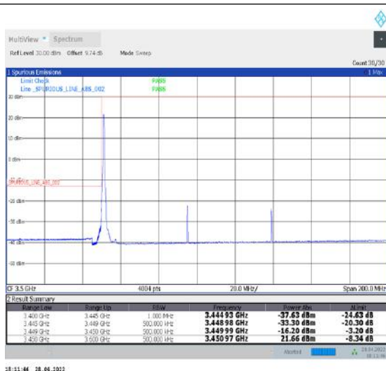
1-N77-3450-3550--30-90-L-4-CP-QPSK-Edge_1RB_Left-1@0-Ant2-PASS-see graph
