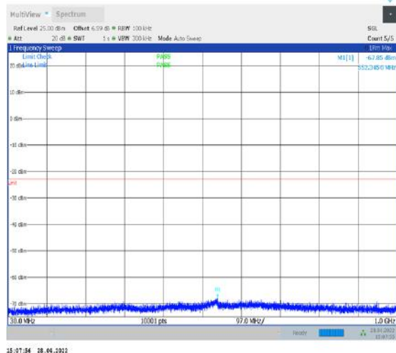
1-N77-3450-3550--30-100-L-1-DFT-QPSK- Edge_1RB_Left-1@0-30-1000-Ant1--67.85--23- PASS
