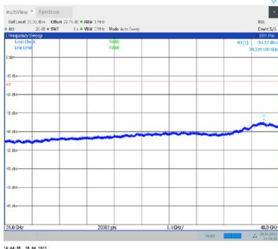
1-N77-3450-3550--30-100-L-1-DFT-QPSK- Edge_1RB_Left-1@0-26000-40000-Ant2--34.37--13- PASS
