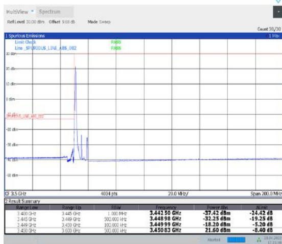
1-N77-3450-3550--30-10-L-4-CP-QPSK-Edge_1RB_Left-1@0-Ant2-PASS-see graph
