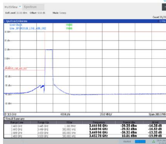
1-N77-3450-3550--30-10-L-6-CP-QPSK-Outer_Full-24@0-Ant2-PASS-see graph
