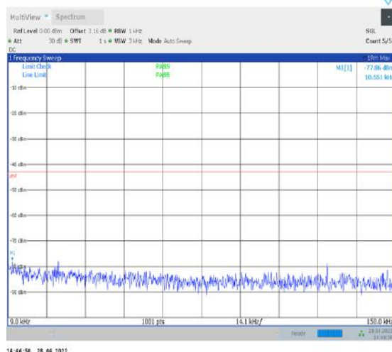
1-N77-3450-3550--30-100-M-1-DFT-QPSK- Edge_1RB_Left-1@0-0.009-0.15-Ant2--77.86--43- PASS
