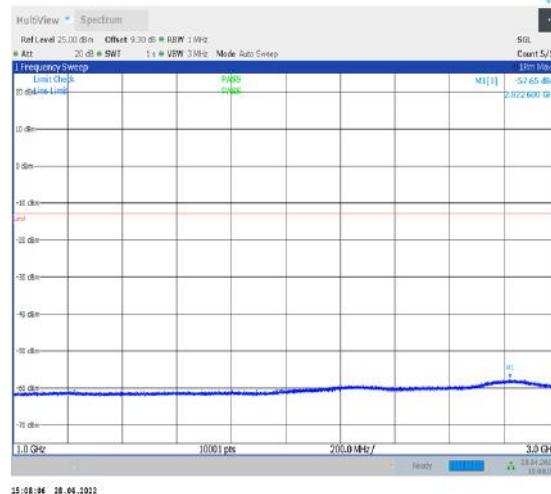
1-N77-3450-3550--30-100-L-1-DFT-QPSK- Edge_1RB_Left-1@0-1000-3000-Ant1--57.65--13- PASS
