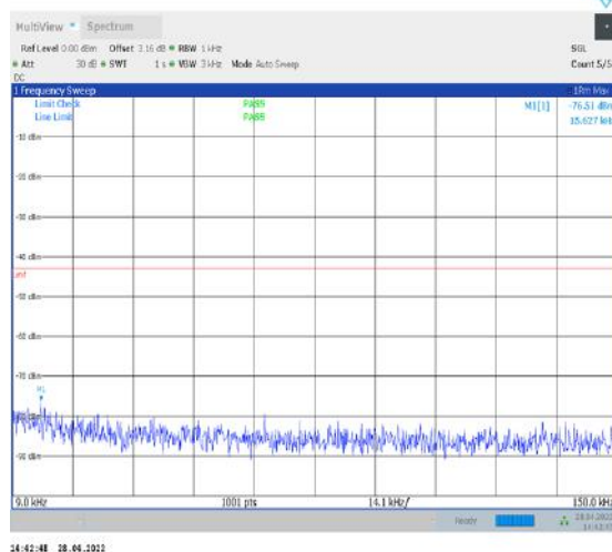
1-N77-3450-3550--30-100-M-1-DFT-QPSK- Edge_1RB_Left-1@0-0.009-0.15-Ant1--76.51--43- PASS
