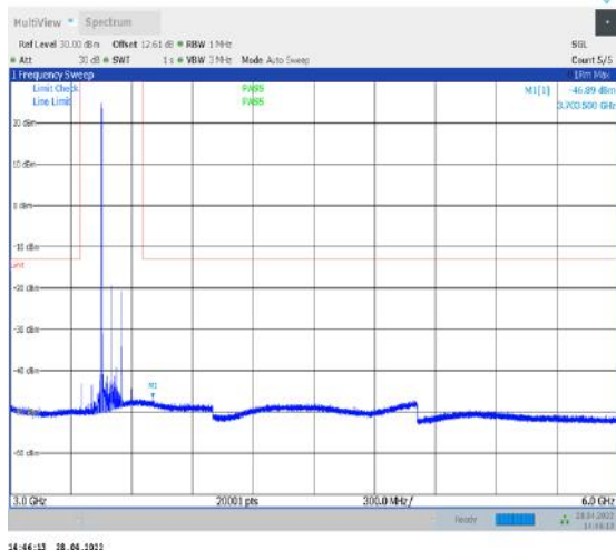
1-N77-3450-3550--30-100-L-1-DFT-QPSK- Edge_1RB_Left-1@0-3000-6000-Ant2--46.89--13- PASS
