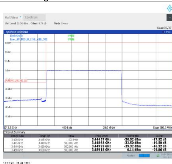
1-N77-3450-3550--30-90-L-6-CP-QPSK-Outer_Full-245@0-Ant2-PASS-see graph
