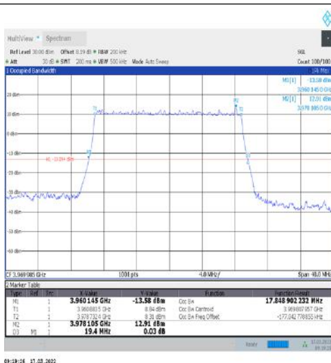
1-N77-3700-3980-30-20-H-5-DFT-256QAM-Outer_Full-50@0-Ant1-17.849-19.400-≤20-PASS
