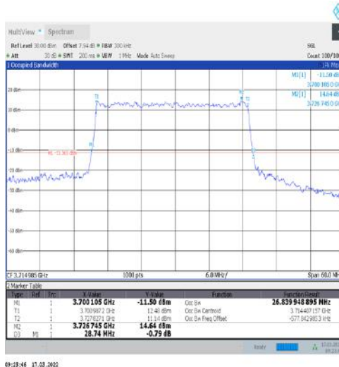
1-N77-3700-3980-30-30-L-3-DFT-16QAM-Outer_Full-75@0-Ant1-26.84-28.740-≤30-PASS
