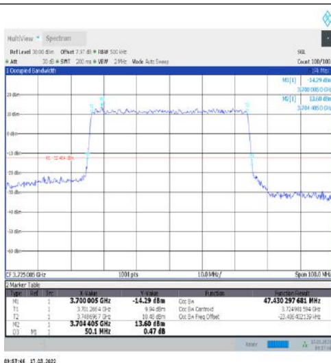
1-N77-3700-3980-30-50-L-6-CP-QPSK-Outet_Full-133@0-Ant1-47.43-50.100-≤50-PASS
