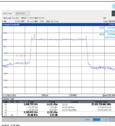
1-N77-3700-3980-30-60-L-7-CP-16QAM-Outer_Full- 162@0-Ant1-57.852-60.480-≤60-PASS
