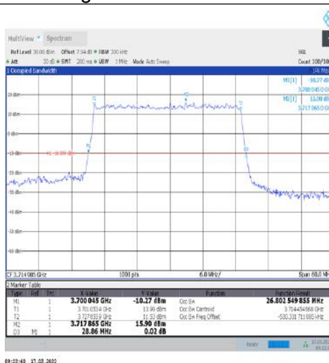
1-N77-3700-3980-30-30-L-1-DFT-QPSK-Outer_Full-75@0-Ant1-26.803-28.860-≤30-PASS
