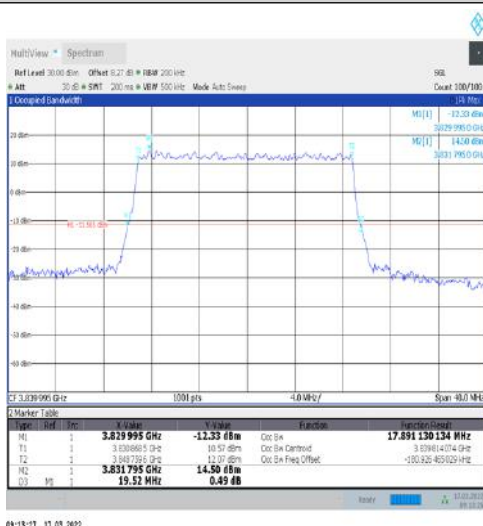
1-N77-3700-3980-30-20-M-4-DFT-64QAM-Outer_Full-50@0-Ant1-17.891-19.520-≤20-PASS
