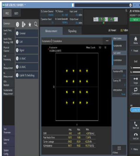
1-N77-3700-3980-30-100-M-7-CP-16QAM-Outer_Full-273@0-Ant1-see graph-PASS
