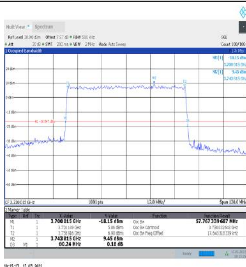
1-N77-3700-3980-30-60-L-9-CP-256QAM- Outer Full-162@0-Ant1-57.767-60.240-≤60-PASS
