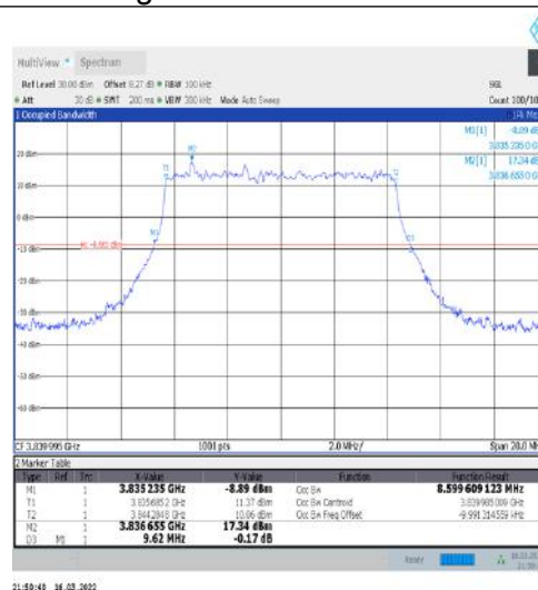
1-N77-3700-3980-30-10-M-1-DFT-QPSK-Outer_Full-24@0-Ant1-8.6-9.620-≤10-PASS
