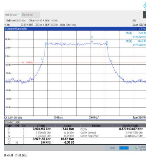
1-N77-3700-3980-30-10-H-2-DFT-P12BPSK-Outer_Full-24@0-Ant1-8.58-9.600-≤10-PASS
