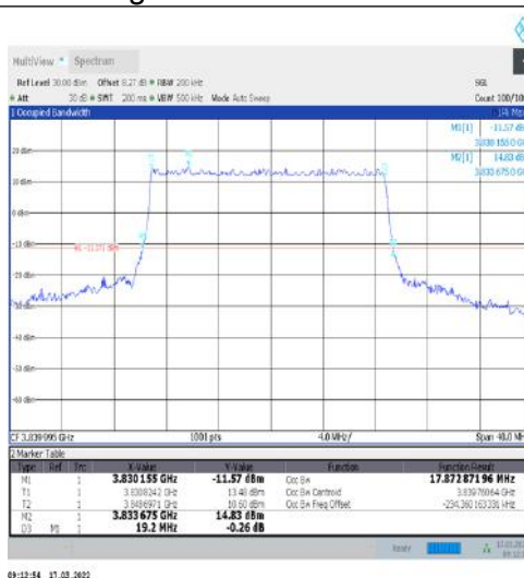
1-N77-3700-3980-30-20-M-3-DFT-16QAM-Outer_Full-50@0-Ant1-17.873-19.200-≤20-PASS
