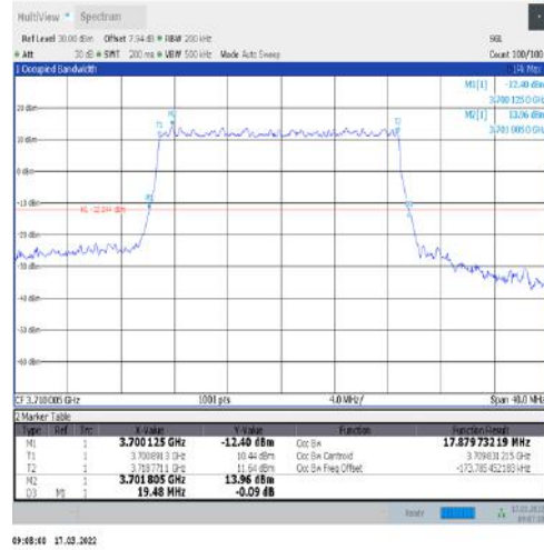
1-N77-3700-3980-30-20-L-4-DFT-64QAM-Outer_Full-50@0-Ant1-17.88-19.480-≤20-PASS
