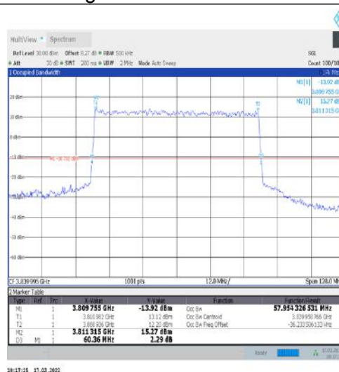
1-N77-3700-3980-30-60-M-3-DFT-16QAM-Outer_Full-162@0-Ant1-57.954-60.360-≤60-PASS
