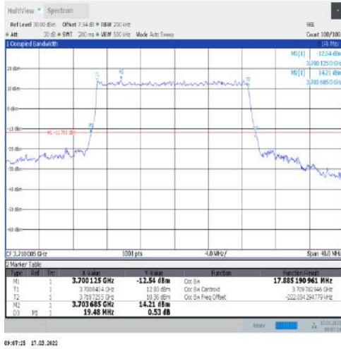
1-N77-3700-3980-30-20-L-3-DFT-16QAM-Outer_Full-50@0-Ant1-17.885-19.480-≤20-PASS
