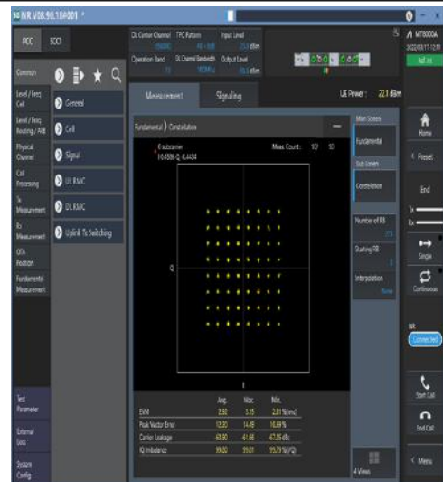
1-N77-3700-3980-30-100-M-8-CP-64QAM-Outer_Full-273@0-Ant1-see graph-PASS
