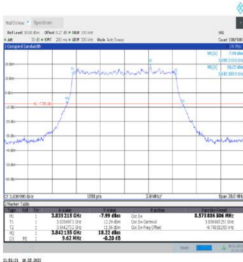
1-N77-3700-3980-30-10-M-2-DFT-PI2BPSK-Outer_Full-24@0-Ant1-8.576-9.620-≤10-PASS
