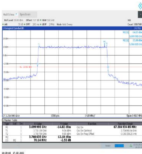
1-N77-3700-3980-30-70-L-6-CP-QPSK-Outer_Full-189@0-Ant1-67.585-70.140-≤70-PASS
