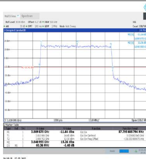
1-N77-3700-3980-30-60-M-1-DFT-QPSK-Outer_Full- 162@0-Ant1-57.796-60.360-≤60-PASS
