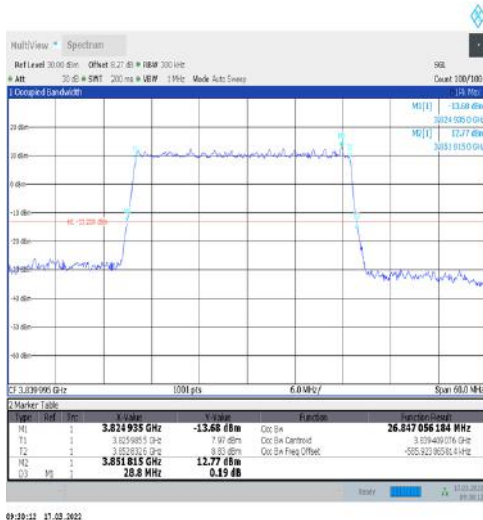
1-N77-3700-3980-30-30-M-5-DFT-256QAM-Outer_Full-75@0-Ant1-26.847-28.800-≤30-PASS
