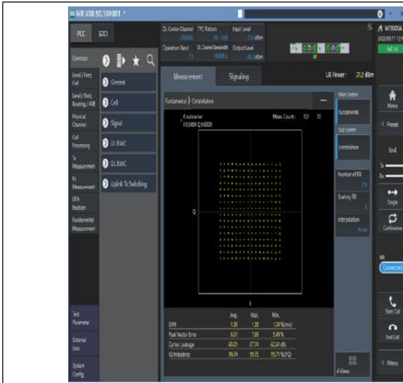
1-N77-3700-3980-30-100-M-5-DFT-256QAM-Outer_Full-270@0-Ant1-see graph-PASS
