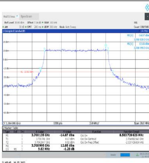
1-N77-3700-3980-30-10-L-7-CP-16QAM-Outer_Full-24@0-Ant1-8.584-9.820-≤10-PASS
